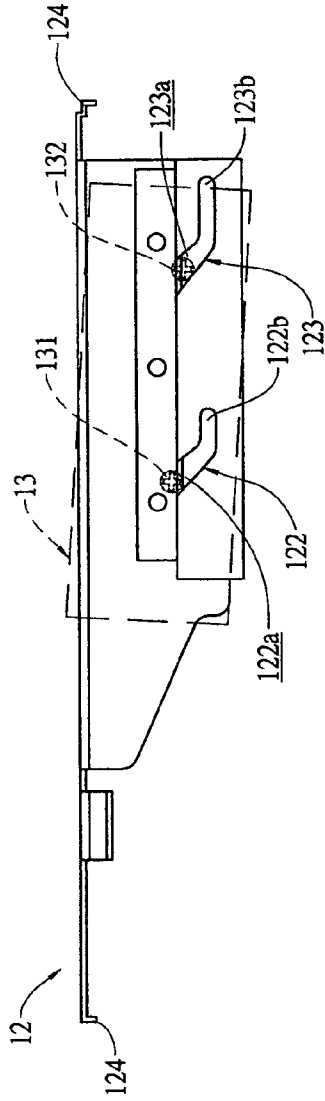
FIG 2 (PRIOR ART)
