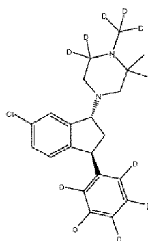
(1 R , 3 S ) - (VI)
