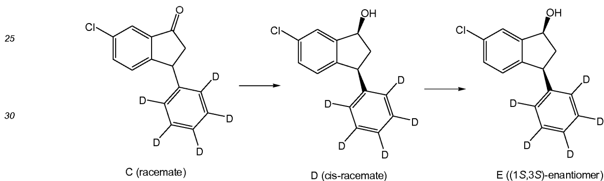
20 Scheme 2. Exemplary synthesis of intermediate E.
