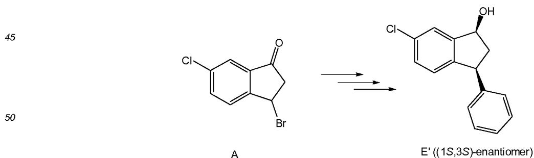
40 Scheme 3. Exemplary synthesis of intermediate E'
