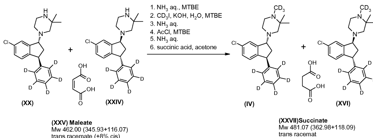
Scheme 17: Synthesis of rac-trans-1-(6-chloro-3-phenyl( d 5 )-indan-1-yl)-1( d 3 ), 2,2-trimethyl-piperazine succinate
