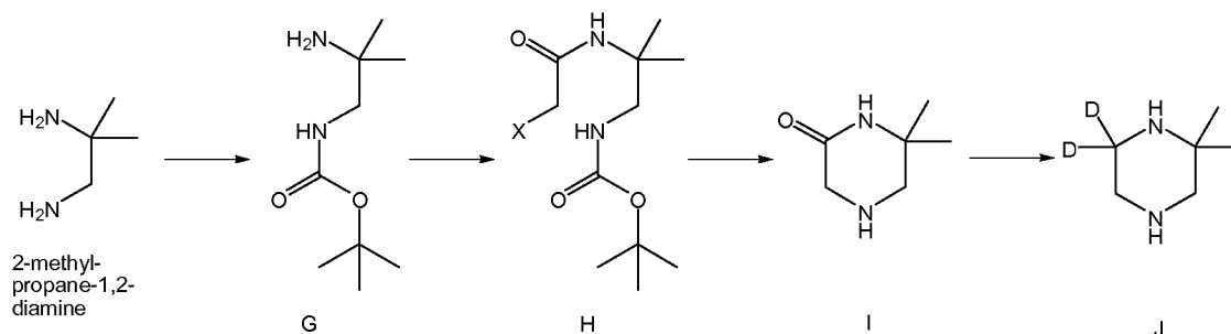
Scheme 6. Exemplary synthesis of intermediate J.
