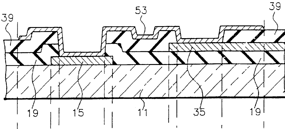
FIG. 1B CONVENTIONAL ART
