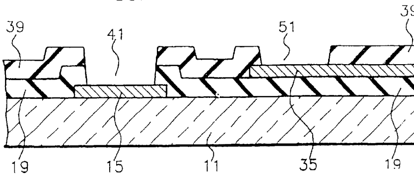
FIG. 2D CONVENTIONAL ART
