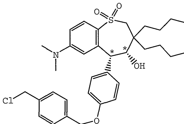
(4R, 5R) - 27
