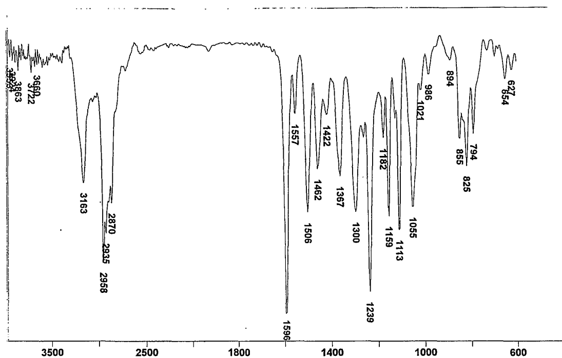
(a) Form I of Compound 41 .
