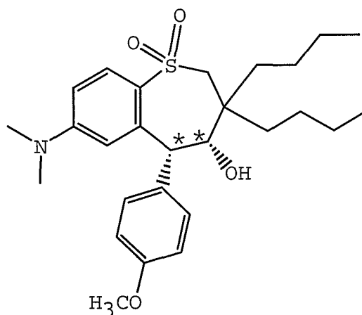
(4R, 5R) - 24
