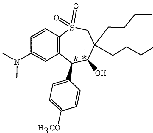
(4S, 5S) - 24
