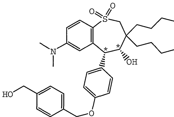
(4R, 5R) - 26
