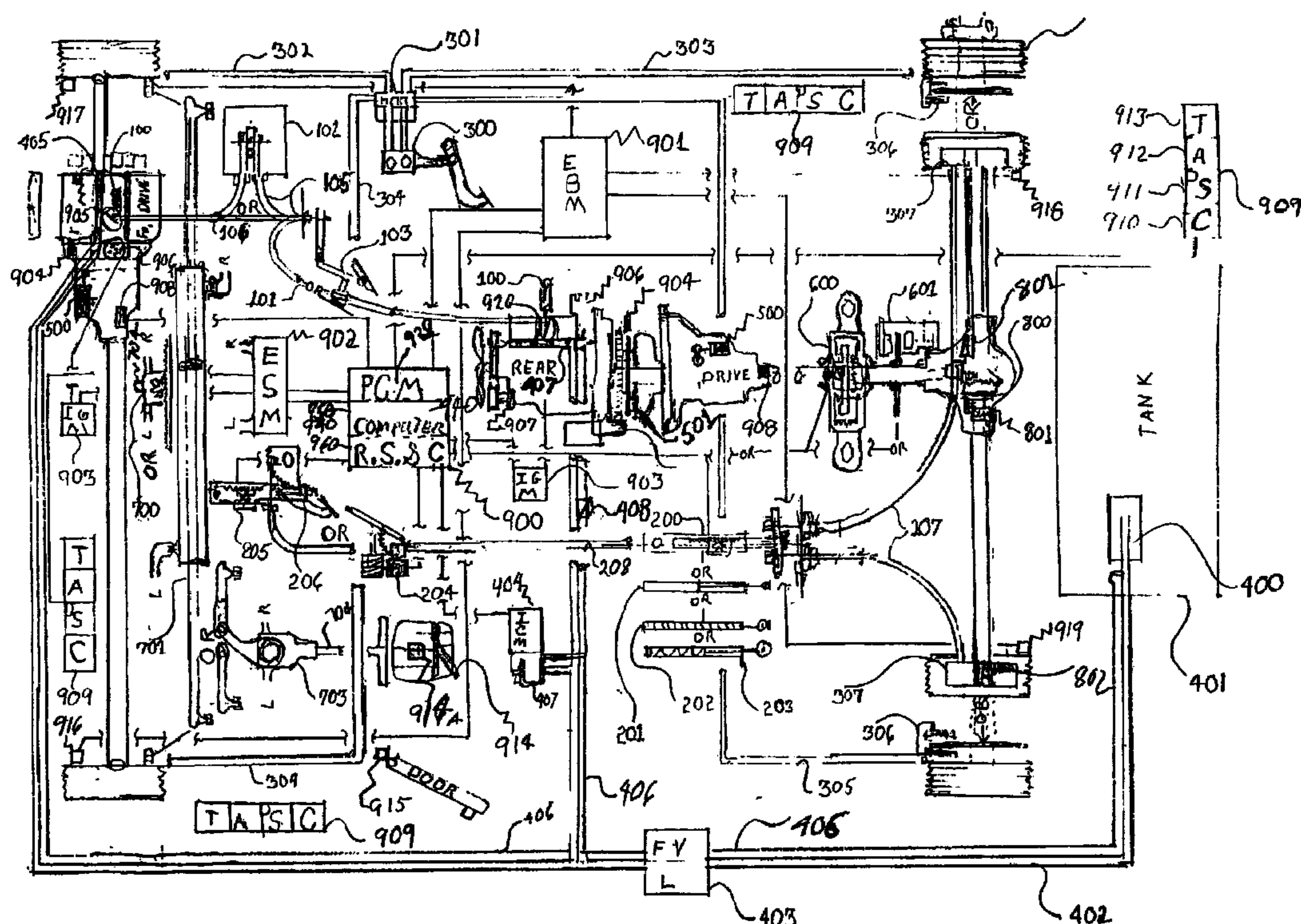
FRONT AND REAR DRIVE AUTOMOBILE COMPONENTS
