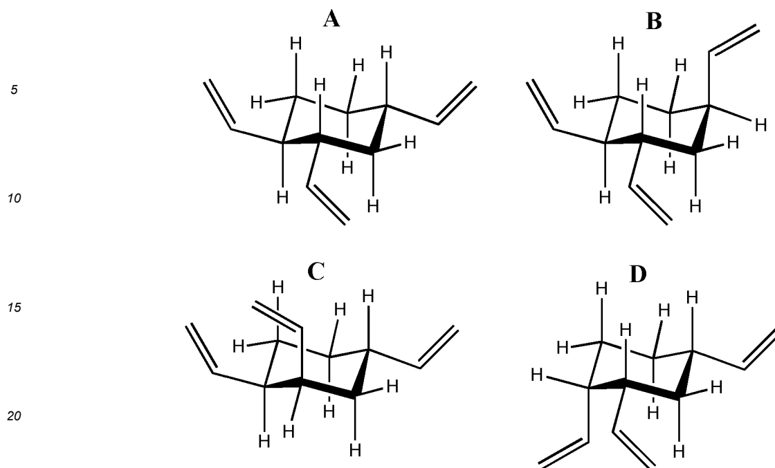
Four Isomeric Forms (A, B, C & D) of 1, 2, 4-Trivinylcyclohexane
