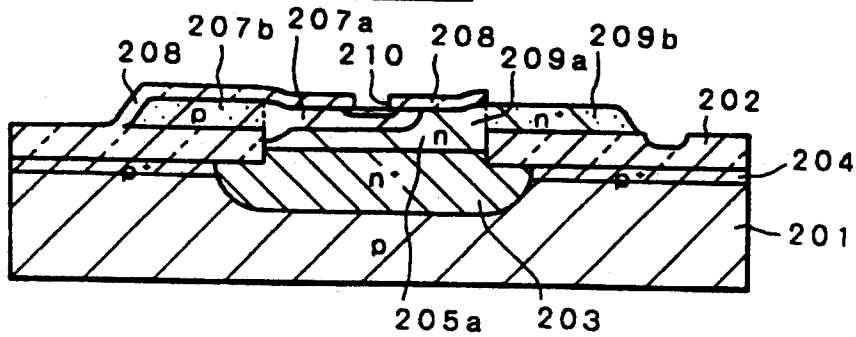
FIG. 1(g) PRIOR ART
