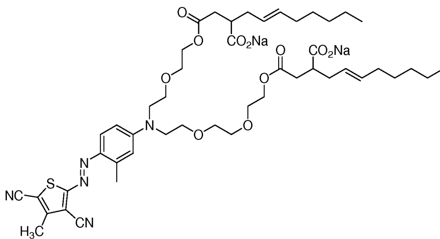
Dye Formula 9
