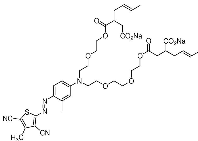
Dye Formula 6
