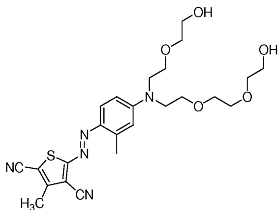
Dye Formula 10
