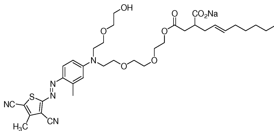
Dye Formula 9
