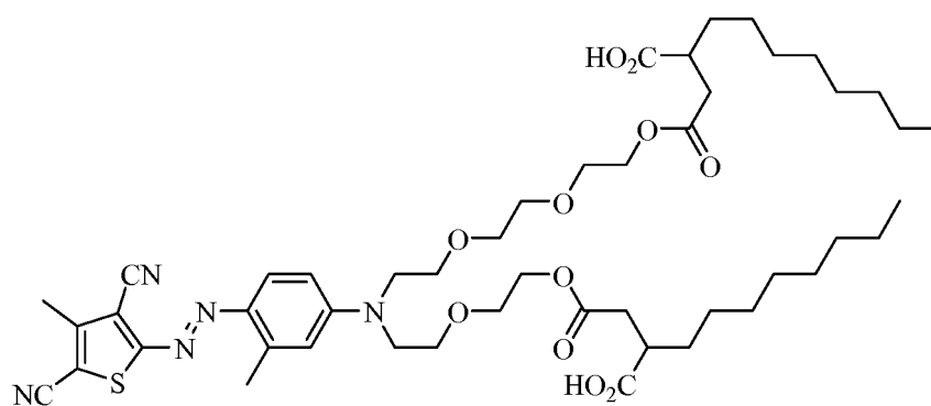
Dye Formula 7
