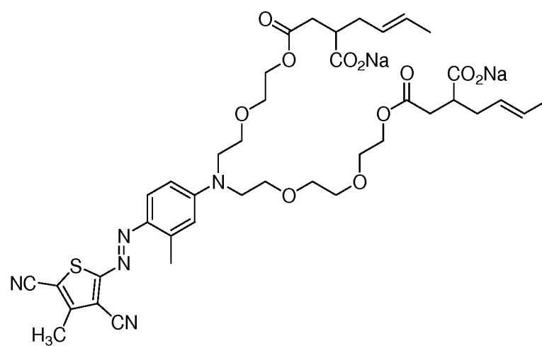
Dye Formula 5
