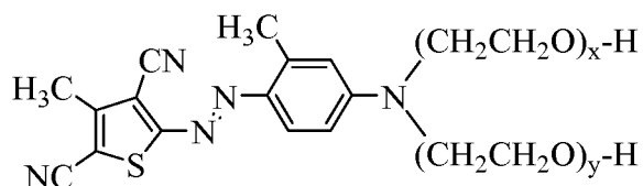
Formula A
