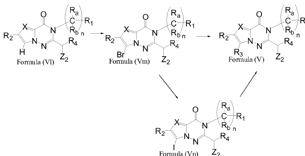
Scheme 14
