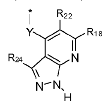
formula (IIIa-6)
