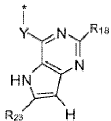
Formel (IIIa-7)
