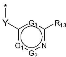
formula (IIb)
