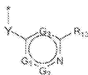
formula (IIb)
