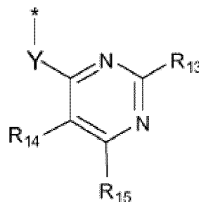
Formel (IIb-2)
