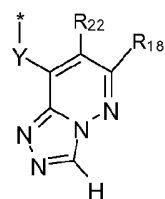
formula (IIIa-20)
