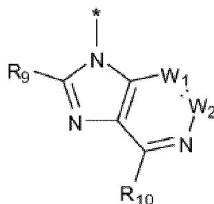
Formel (IIa)
