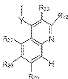
formula (IIIb-1)
