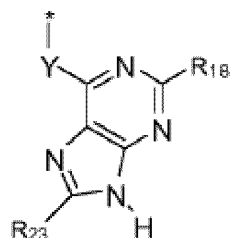
Formel (IIIa-1)
