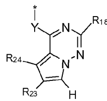
formula (IIIa-15)
