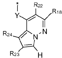
formula (IIIa-16)
