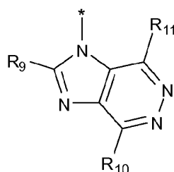
formula (IIa-1)
