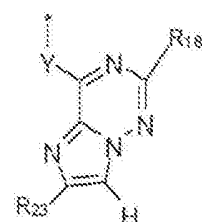
formula (IIa-21)
