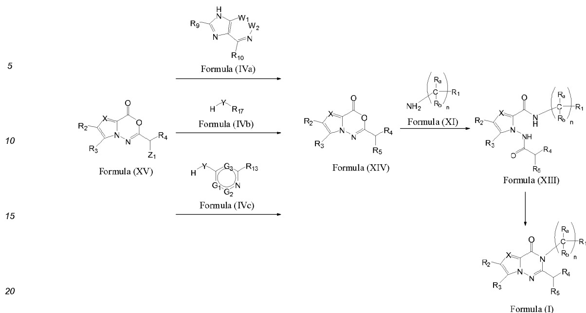
Scheme 5
