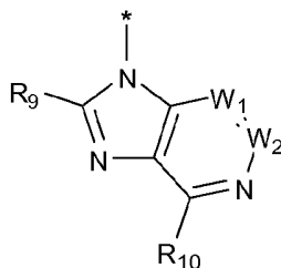
formula (IIa)
