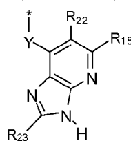
formula (IIIa-2)
