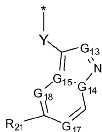
formula (IIId)
