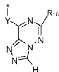
Formel (IIIa-19)
