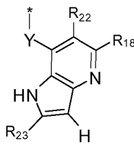
formula (IIIa-8)
