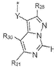
formula (III-d-2)
