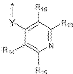
formula (IIb-1)
