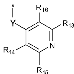
formula (IIb-1)
