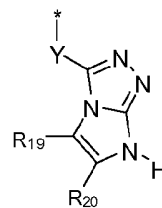
formula (IIIc-2)
