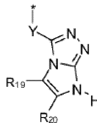
Formel (IIIc-2)
