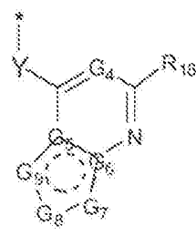
formula (IIla)
