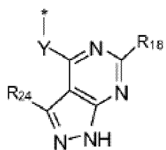
Formel (IIIa-5)
