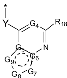
formula (IIIa)
