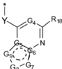
formula (IIIa)
