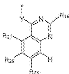
formula (IIIb-2)
