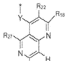
formula (IIIb-5)
