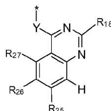
formula (IIIb-2)
