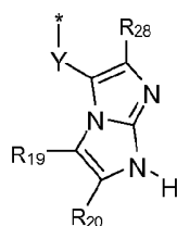
formula (IIIc-1)
