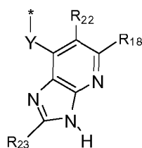
formula (IIIa-2)
