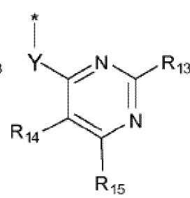
Formel (IIb-2)
