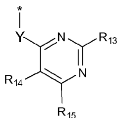
formula (IIb-2)
