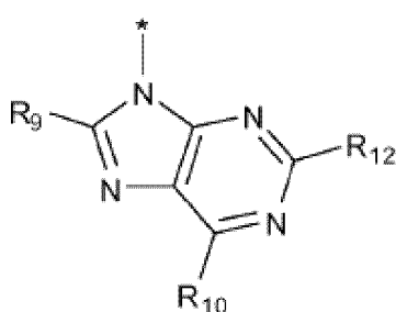
Formel (IIa-2)
