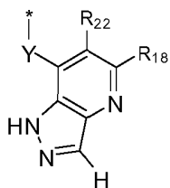
formula (IIIa-10)
