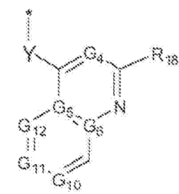
formula (IIlb)
