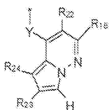
formula (IIa-16)
