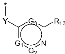
formula (IIb)
