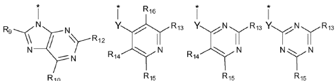
Formel (IIa-2)
