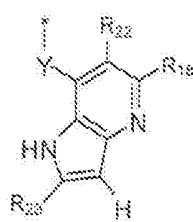
formula (IIa-8)
