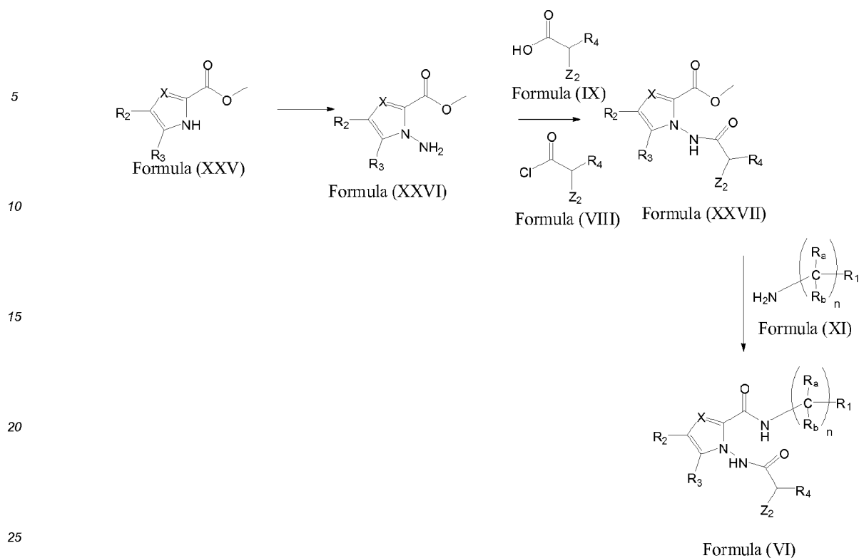
Scheme 11
