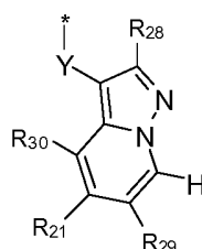
formula (IIId-1)
