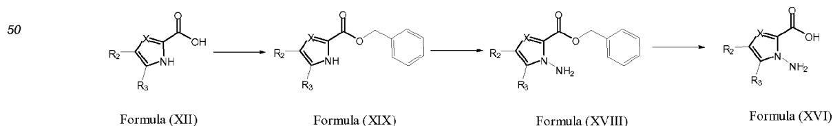
Scheme 7
