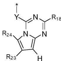
formula (IIIa-11)
