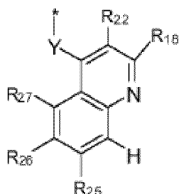
Formel (IIIb-1)
