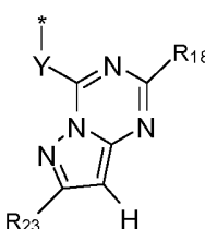
formula (IIIa-13)
