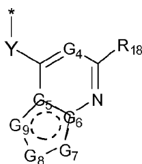
formula (IIIa)
