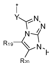
formula (IIIc-2)
