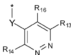
formula (IIb-4)
