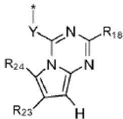
Formel (IIIa-11)
