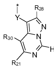
formula (IIId-2)
