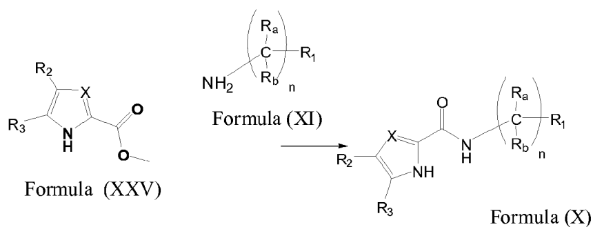
Scheme 10
