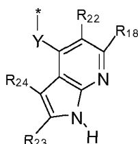
formula (IIIa-4)
