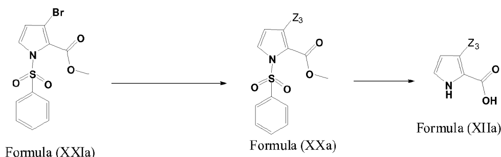
Scheme 8
