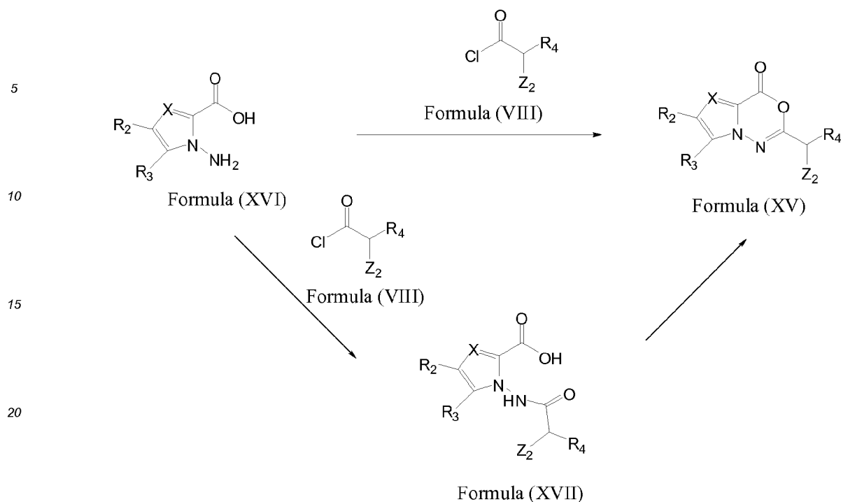
Scheme 6
