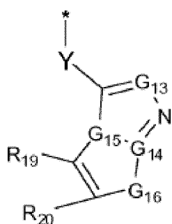
Formel (IIIc)
