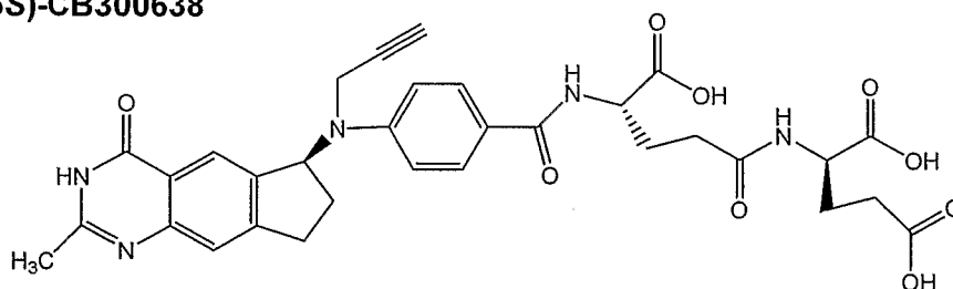
(6S)-CB300638
