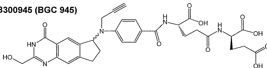
(6S)-CB300945
