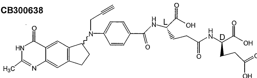
(6S)-CB300638
