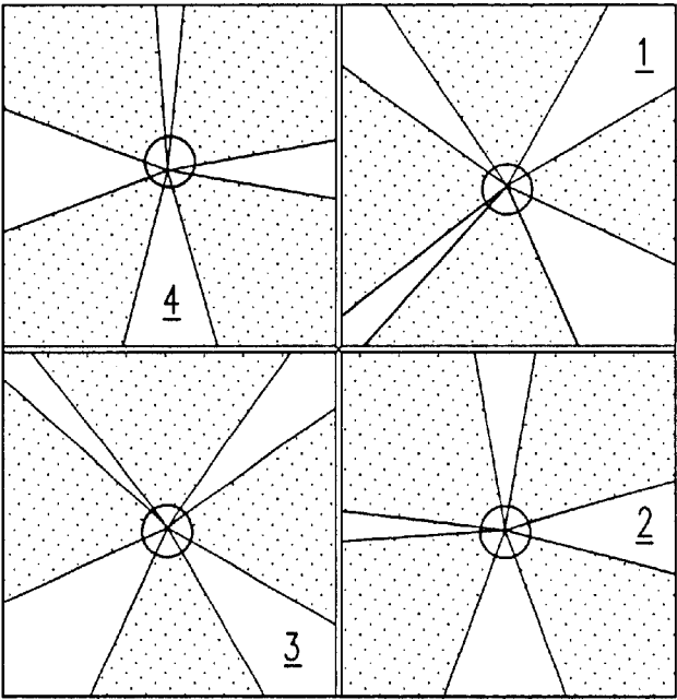
MASKING PATTERN FOR FOUR OPTICAL FIBERS
