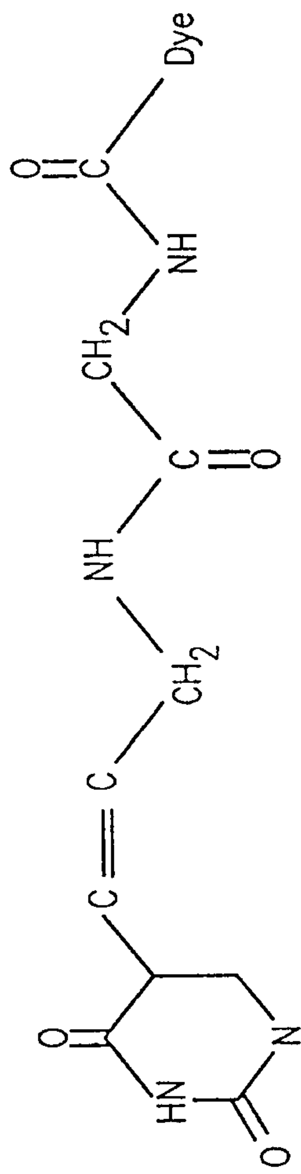
Diglycinylnyl linker
