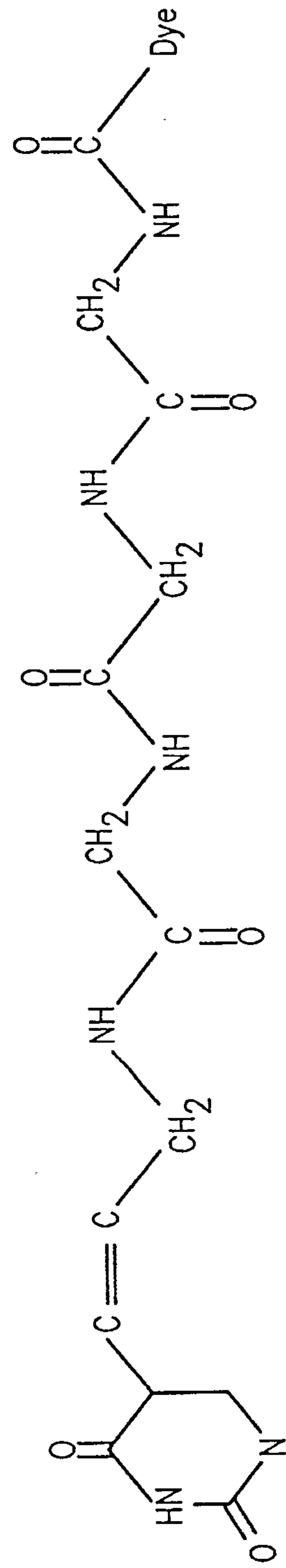
Tetraglycinylnyl linker
