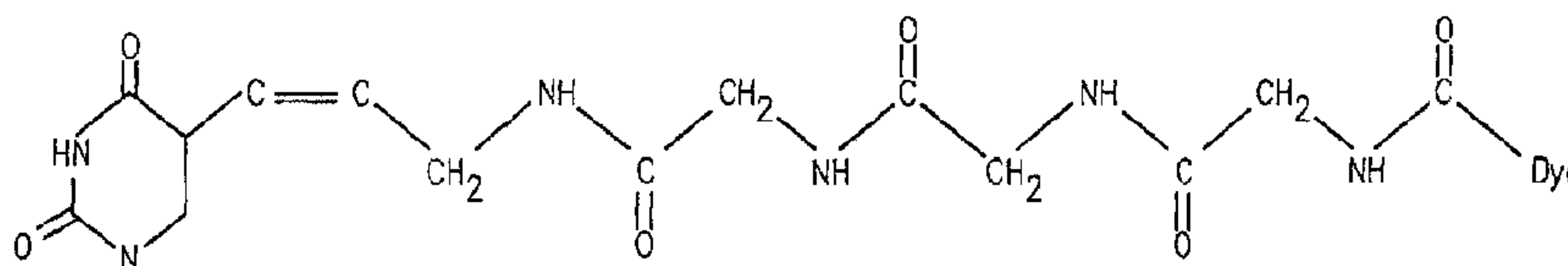
Tetraglycinyll linker
