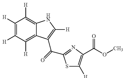
Structural Formula 1
