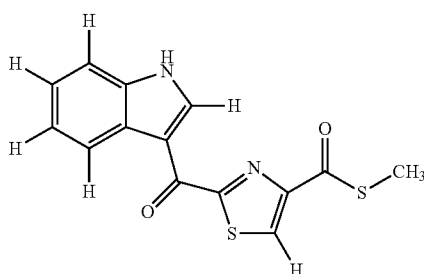
Structural Formula 3
