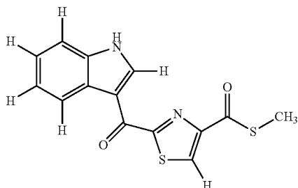
Structural Formula 3
