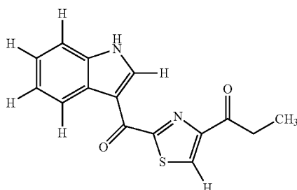
Structural Formula 2
