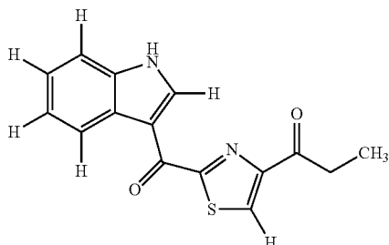
Structural Formula 2
