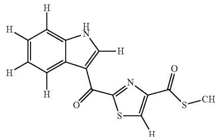
Structural Formula 3
