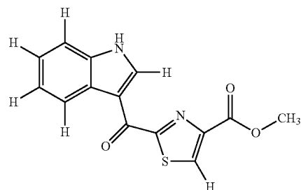
Structural Formula 1
