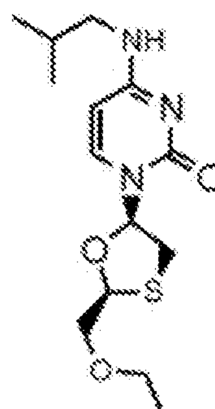
3tc-C6-2,4*,0
