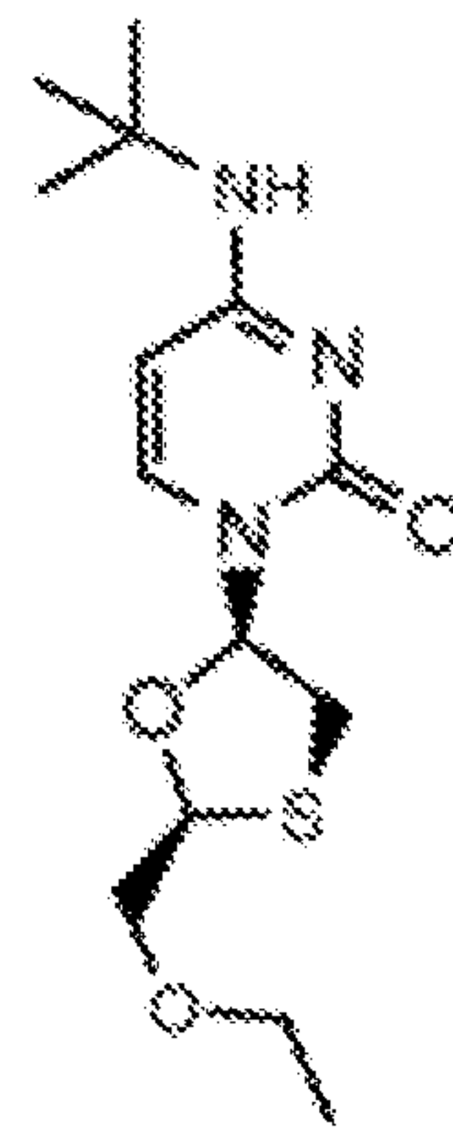
3tc-C6-2,4**,0
