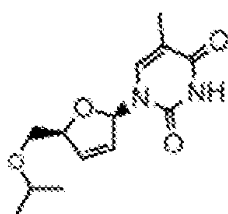
O-isopropyl-d4T
