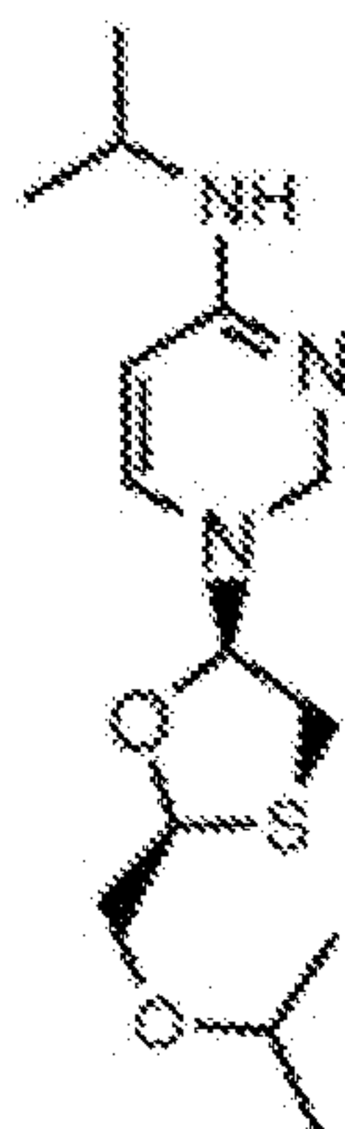
3tc-C6-3*,3*,0
