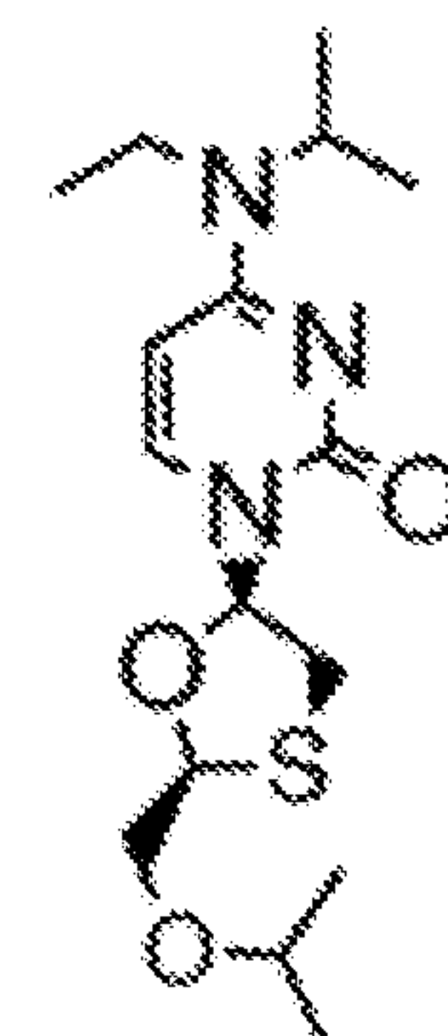
3tc-C8-3',2,3'
