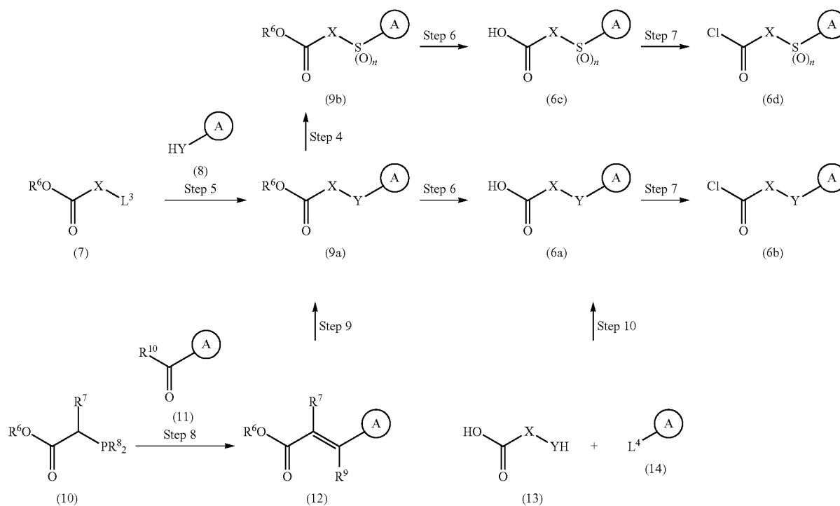
Reaction Scheme 2
