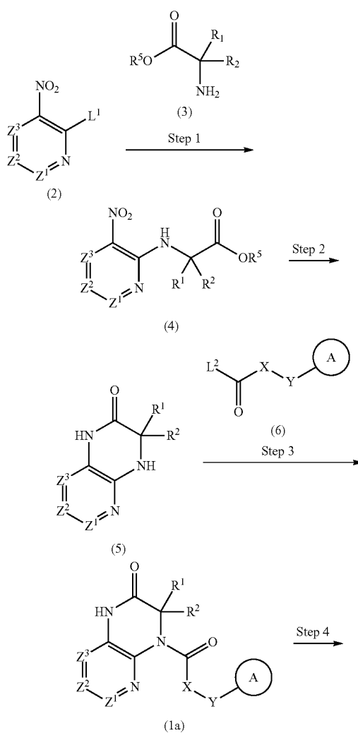
Reaction Scheme 1
