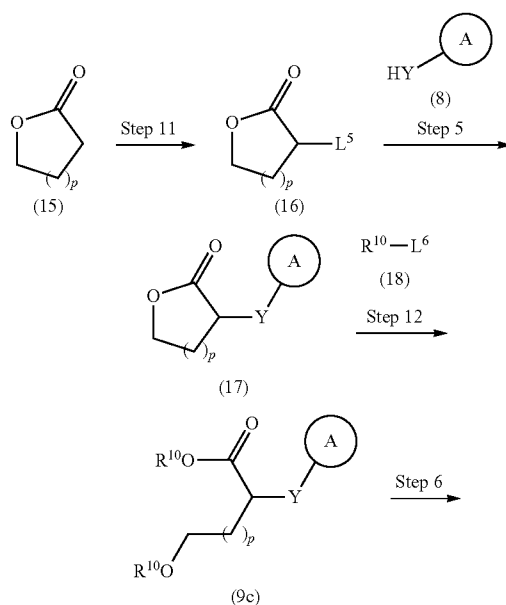
Reaction Scheme 3
