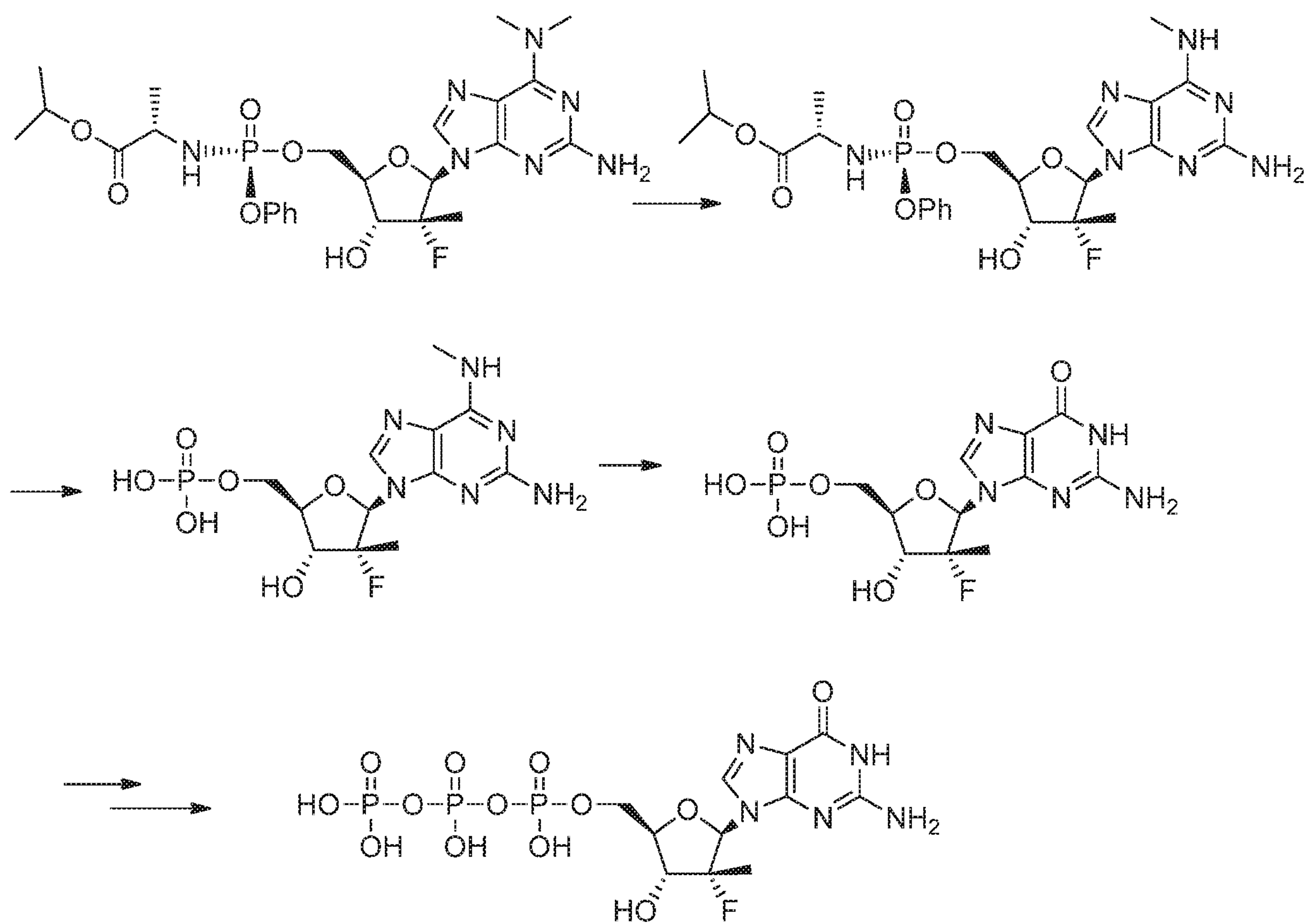
Scheme 2
