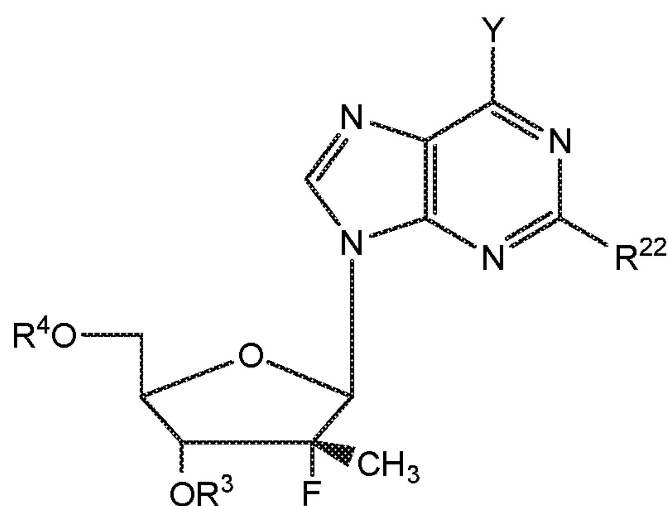
Formula IIa
