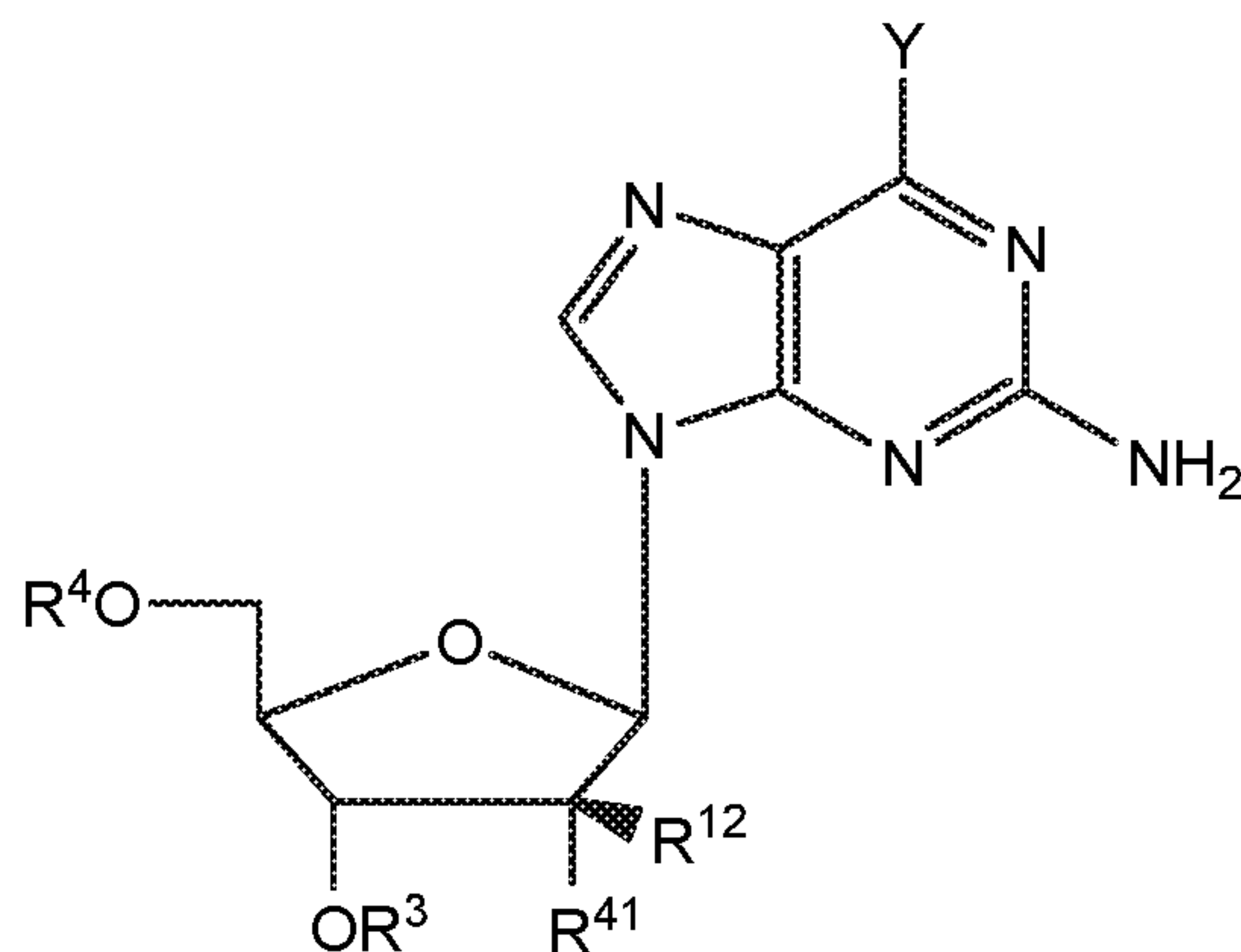
Formula VI
