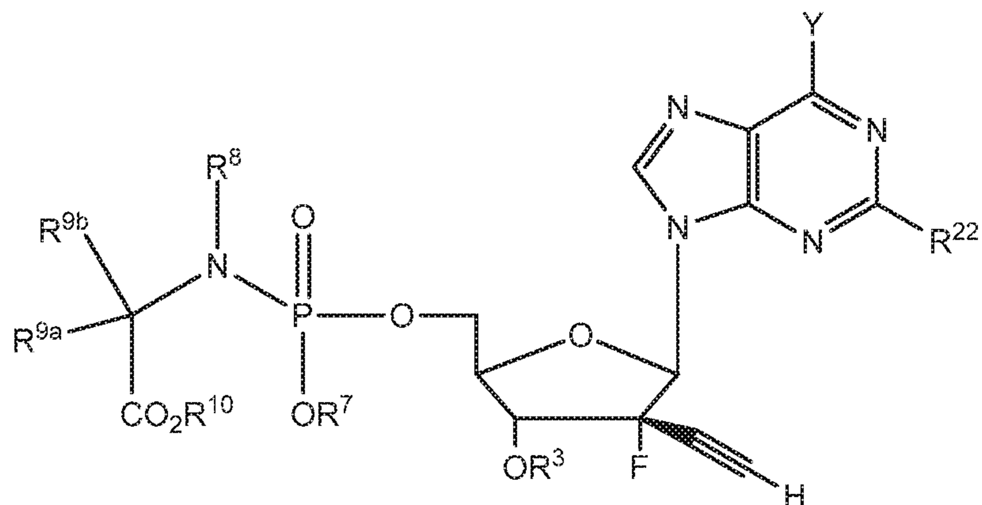
Formula V
