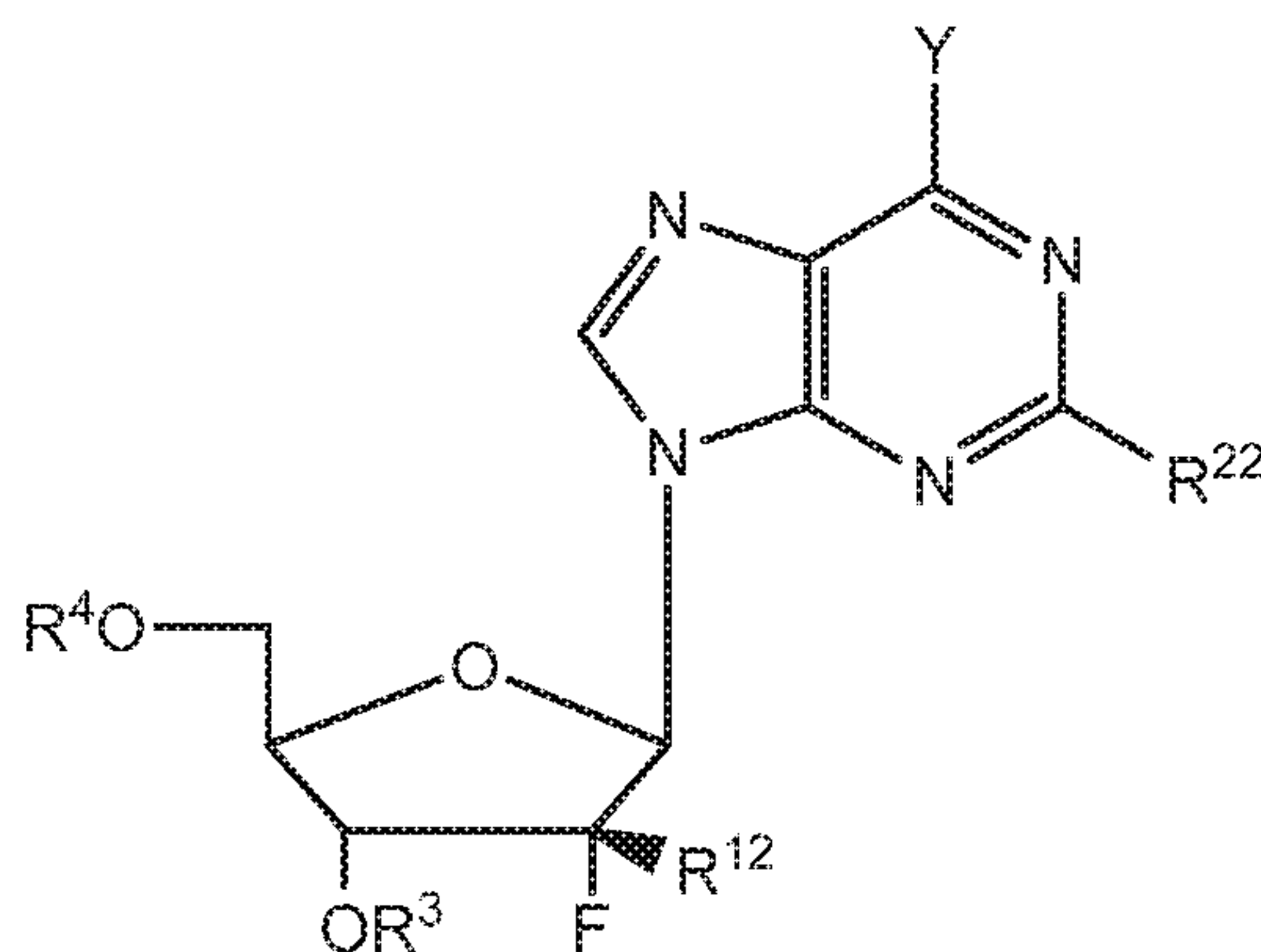
Formula II
