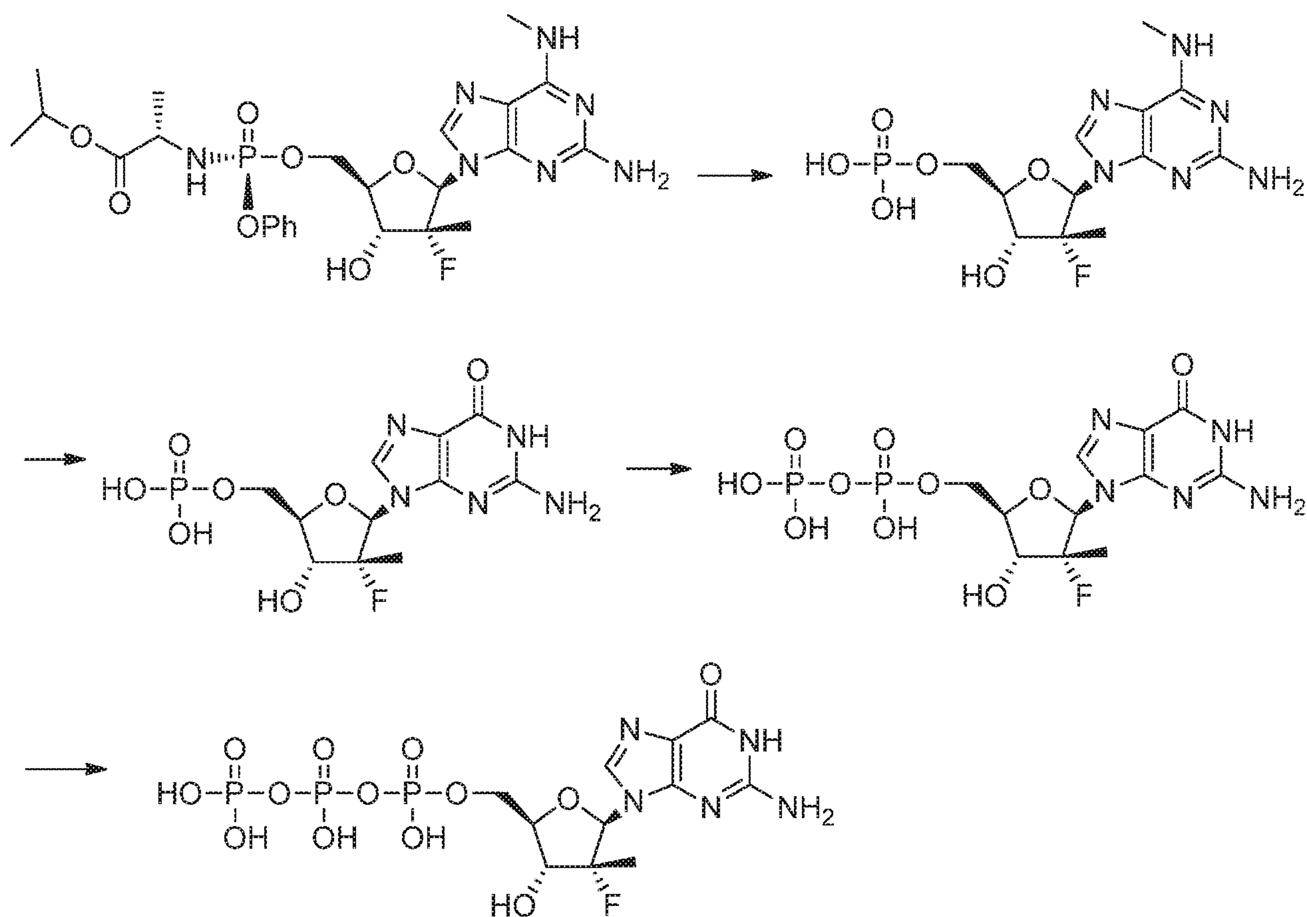
Scheme 1
