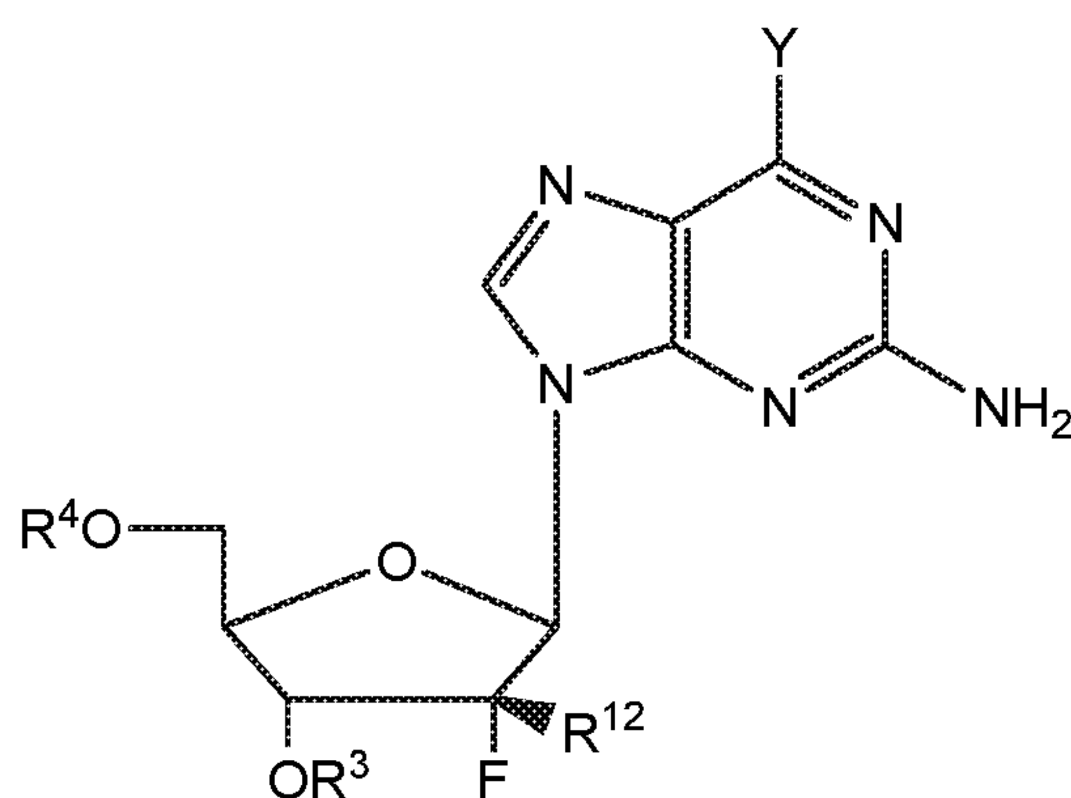
Formula I
