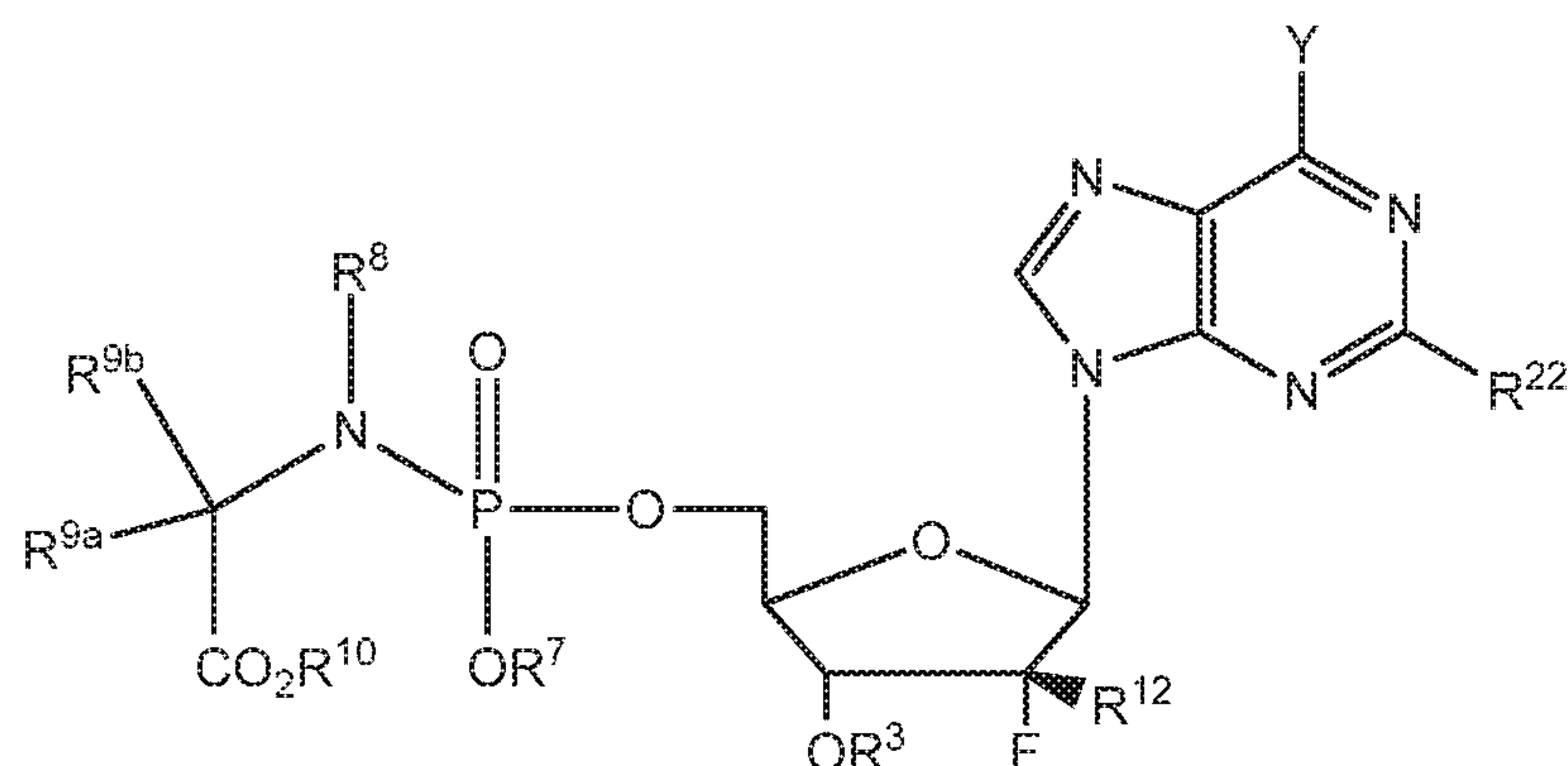
Formula III
