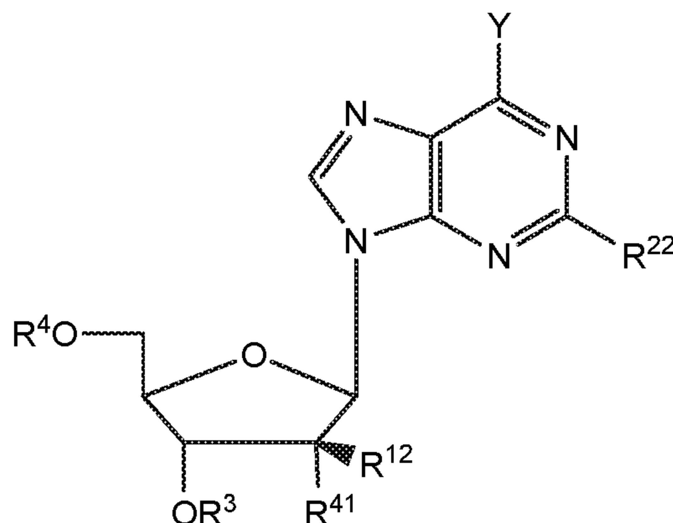
Formula VII
