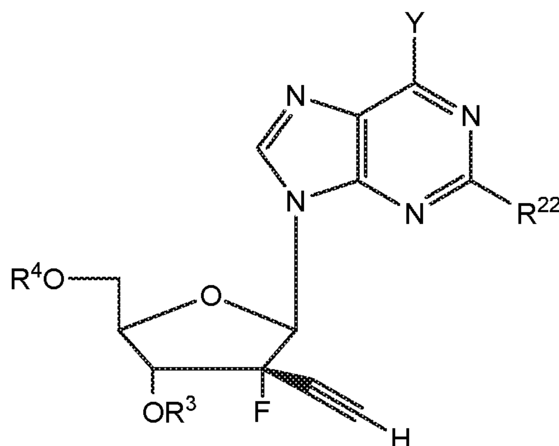
Formula IIb
