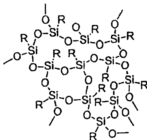
[Chemical formula 5]
