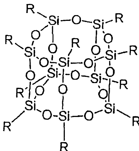
[Chemical formula 7]
