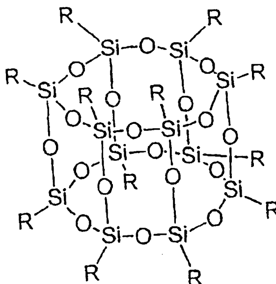
[Chemical formula 8]
