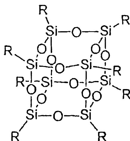
[Chemical formula 6]
