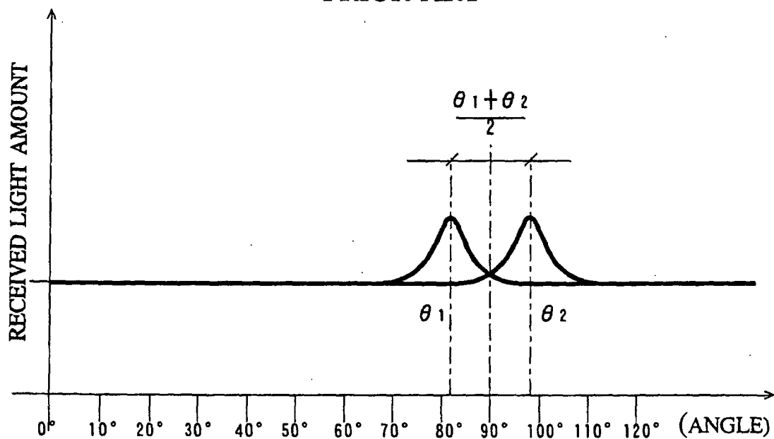
FIG.4 PRIOR ART
