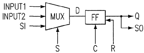
FIG. 4A (PRIOR ART)
