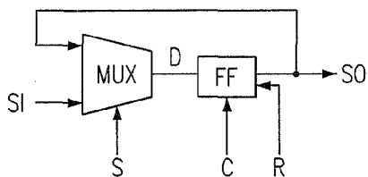
FIG. 4B (PRIOR ART)
