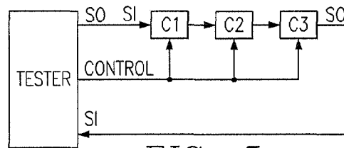
FIG. 5 (PRIOR ART)
