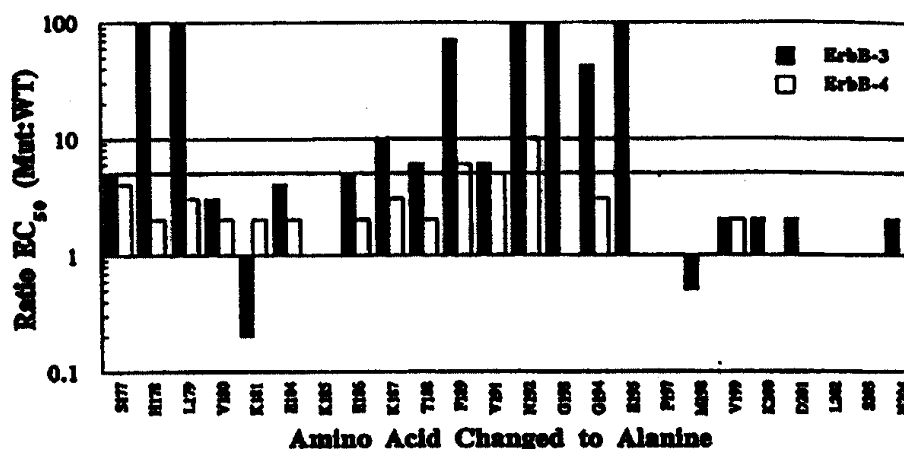
Alanine Scan of HRG EGF-like Domain on ErbB-3 and ErbB-4
