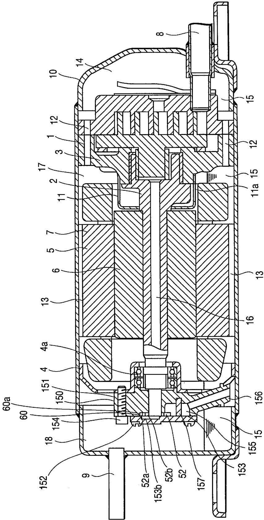
FIG. 14 (PRIOR ART)
