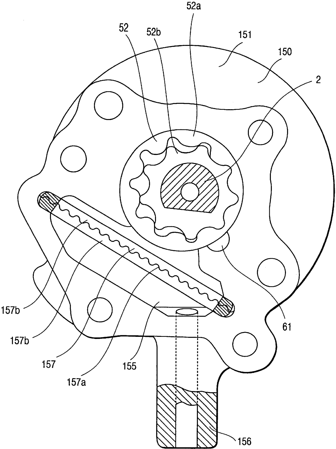
FIG. 15 (PRIOR ART)
