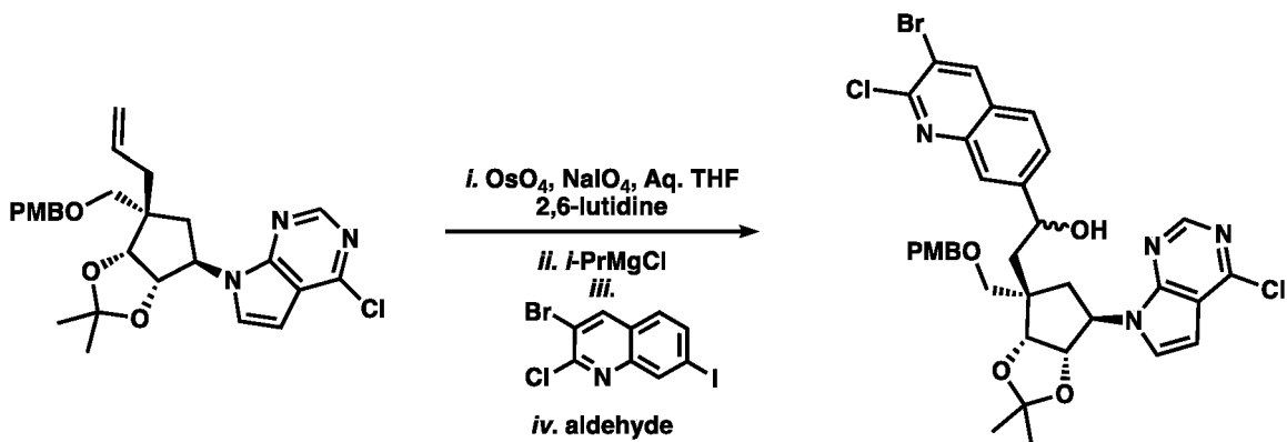
Intermediate 2-10
