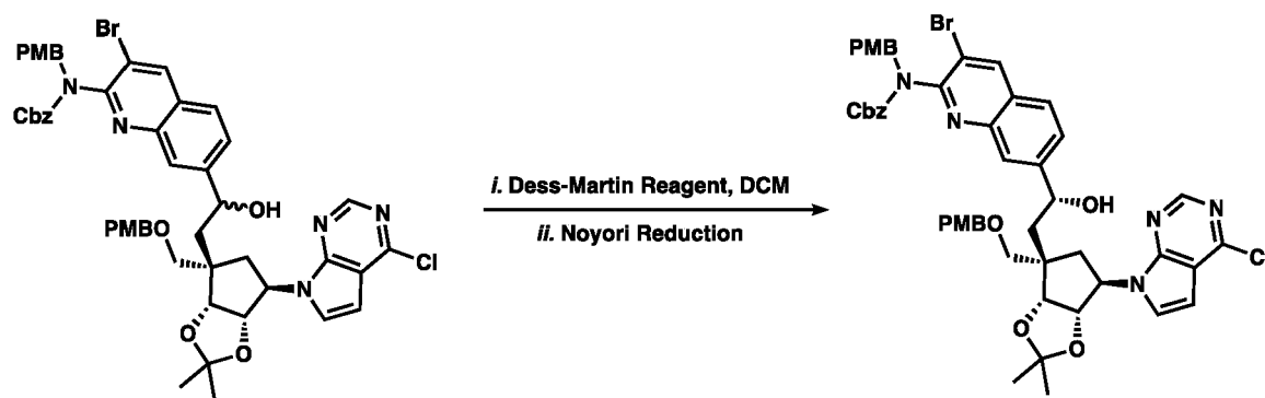
Intermediate 2-8a
