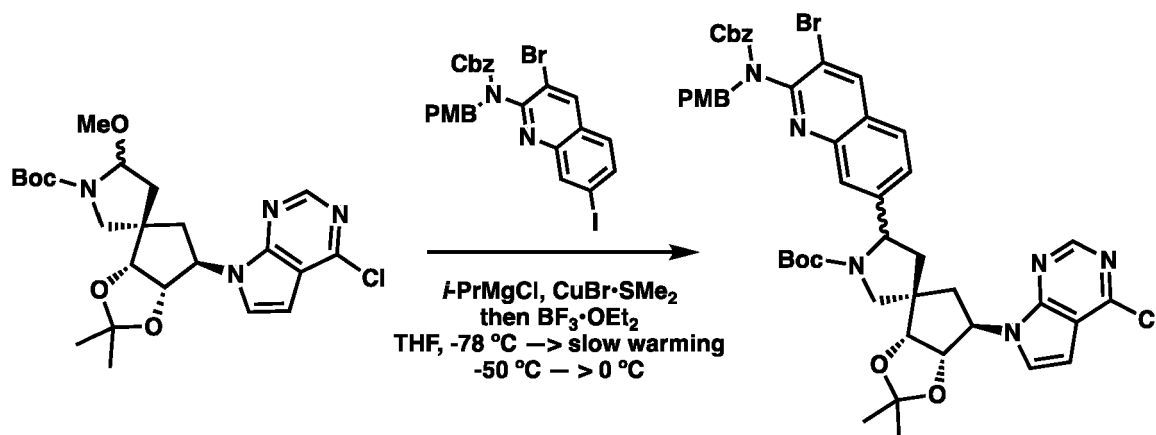
Intermediates 1-8 R&S
