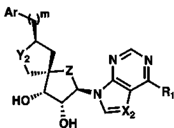
(Formel IIIa)
