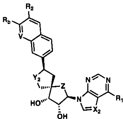
(Formel IVa)
