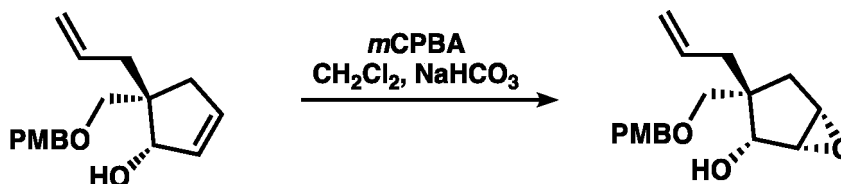
Intermediate 2-5
