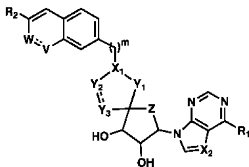
(Formel II)
