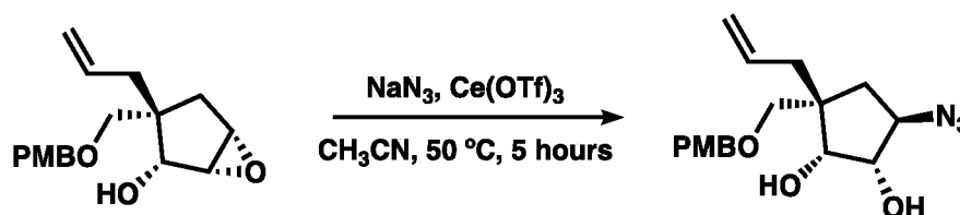
Intermediate 2-6
