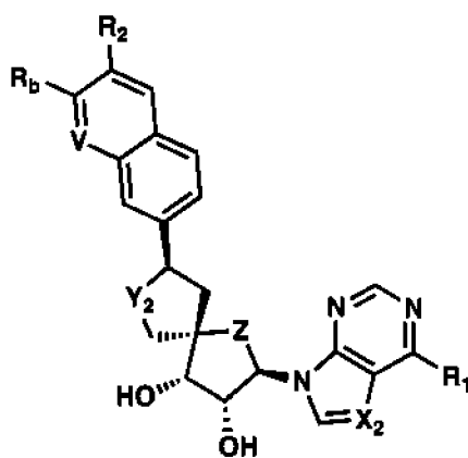
(Formule IVa)
