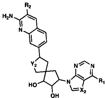
(Formule V)
