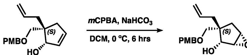
Intermediate 2-5
