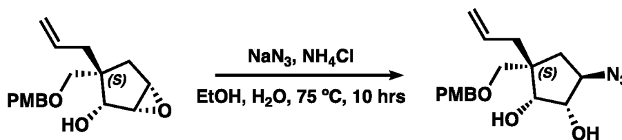
Intermediate 2-6
