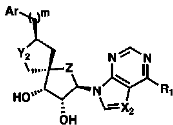
(Formule IIIa)
