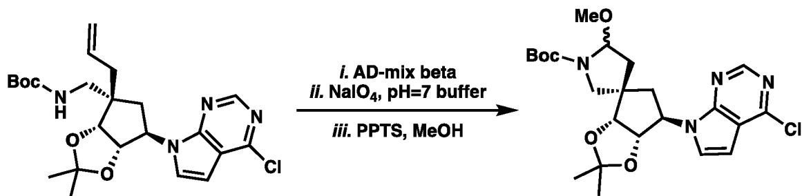
Intermediates 1-6 R&S
