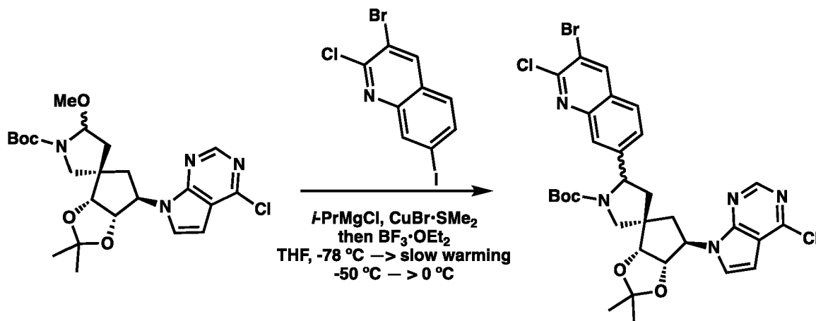
Intermediates 1-7 R&amp;S
