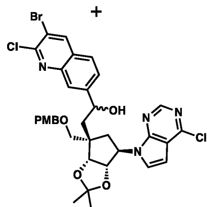
Epi -Intermediate 2-10
