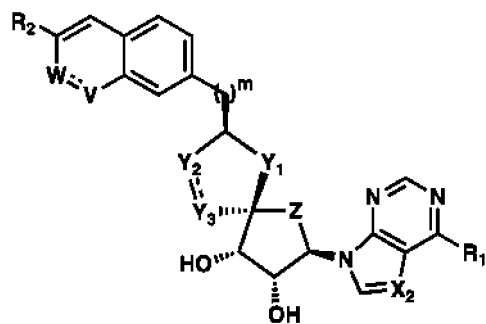
(Formel IIa)
