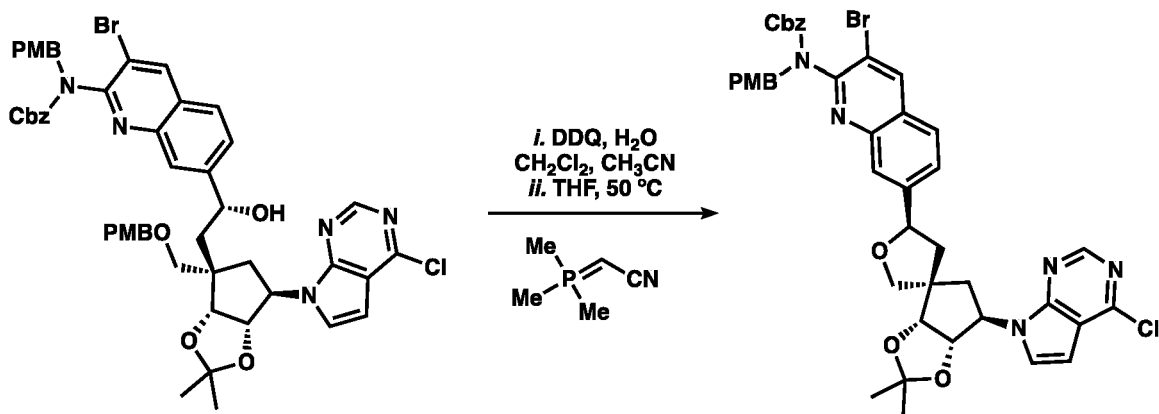
Intermediate 2-8a
