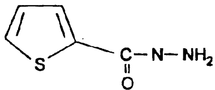
2-TH hydrazine
