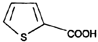
2-TH acid
