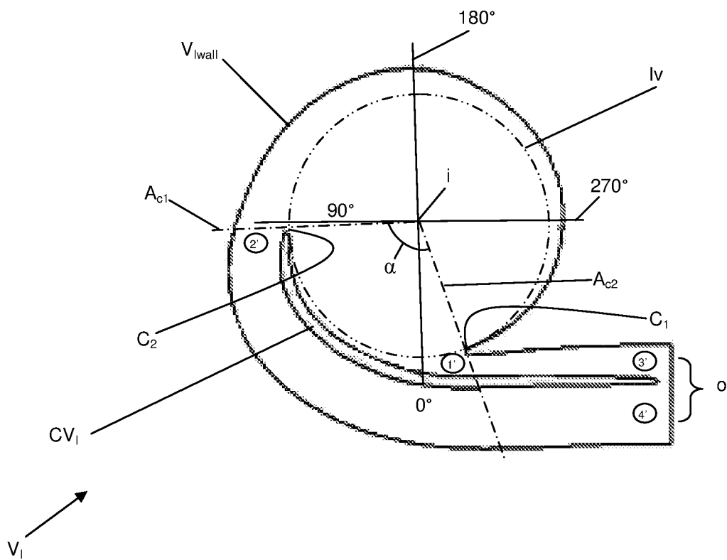
Figure 2: Dual Volute According to the Present Invention
