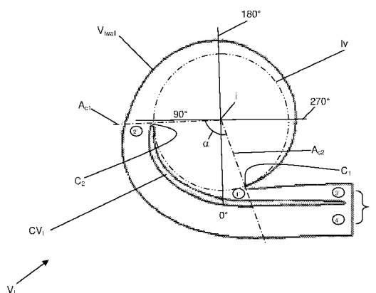
Figure 2: Dual Volute According to the Present Invention
