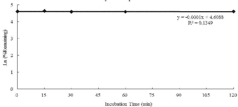
Metabolic Stability of Compound 16 in Mouse Plasma
