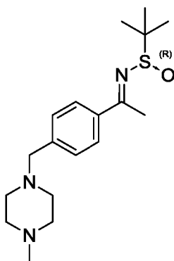
(R S )-2-methyl-N-(1-(4-((4-methylpiperazin-1-yl)methyl)phenyl)ethylidene)propane-2-sulfonamide
