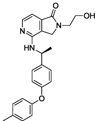
(S)-2-(2-hydroxyethyl)-4-((1-(4-( p -tolyloxy)phenyl)ethyl)amino)-2,3-dihydro-1 H -pyrrolo[3,4- c ]pyridin-1-one
