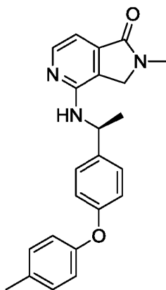
(S)-2-methyl-4-((1-(4-( p -tolylloxy)phenyl)ethyl)amino)-2,3-dihydro-1 H -pyrrolo[3,4- c ]pyridin-1-one
