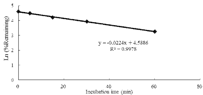
Metabolic Stability of Compound 16 in Human Liver Microsome
