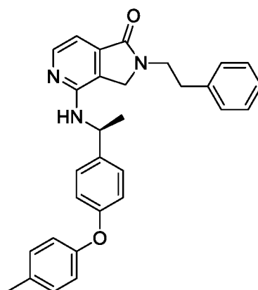
(S)-2-phenethyl-4-((1-(4-( p -tolylloxy)phenyl)ethyl)amino)-2,3-dihydro-1 H -pyrrolo[3,4- c ]pyridin-1-one
