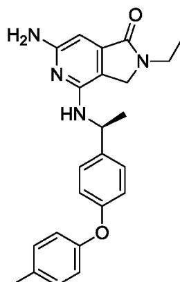
(S)-6-amino-2-ethyl-4-((1-(4-( p -tolylloxy)phenyl)ethyl)amino)-2,3-dihydro-1 H -pyrrolo[3,4- c ]pyridin-1-one
