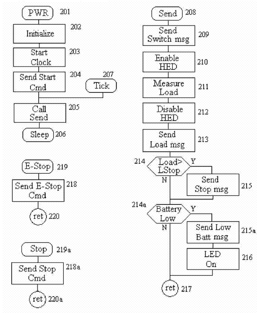
Fig 8 Sender Logic
