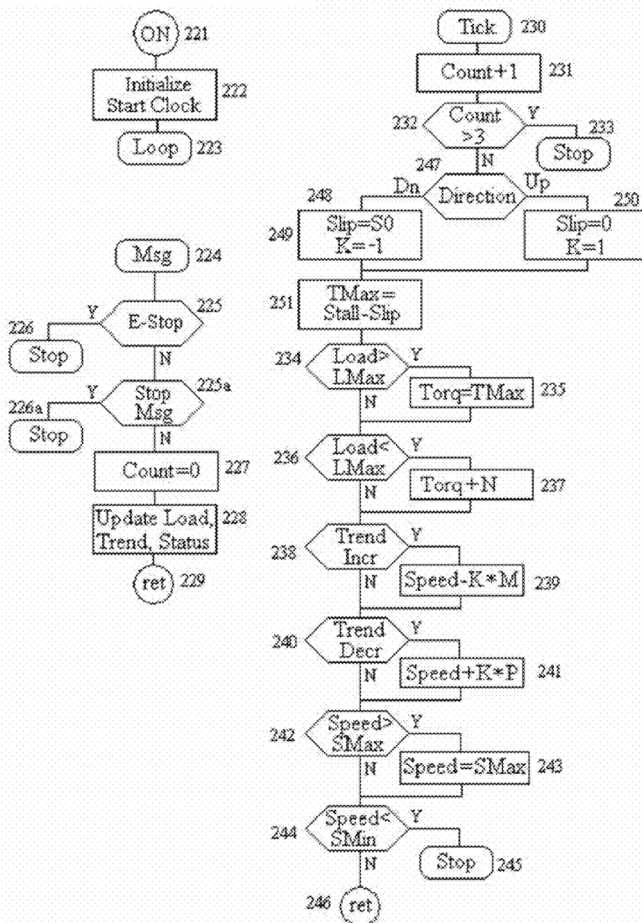
Fig 9 Receiver Logic
