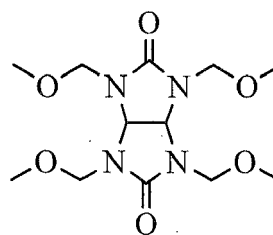
Crosslinker 4
