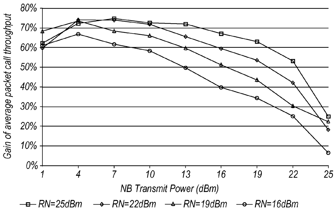
Fig.21B Gain in average packet call throughput for deployment scenario 2.
