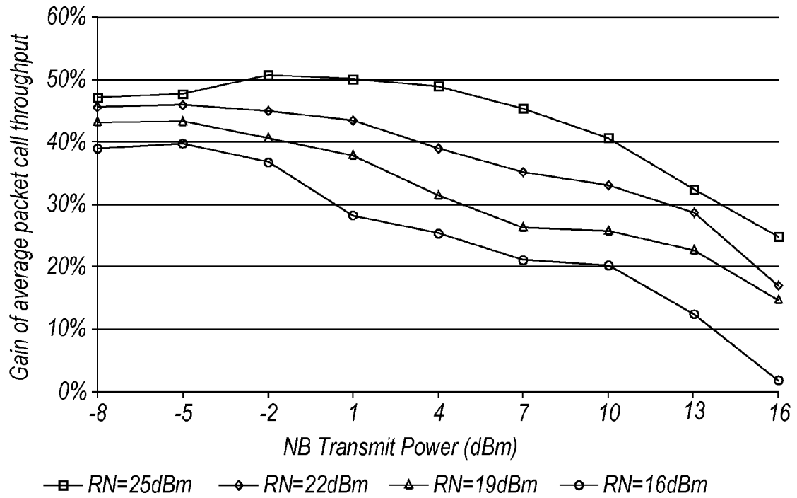
Fig.21A Gain in average packet call throughput for deployment scenario 1.
