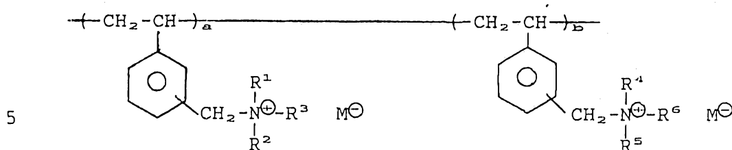
Formula (I)
