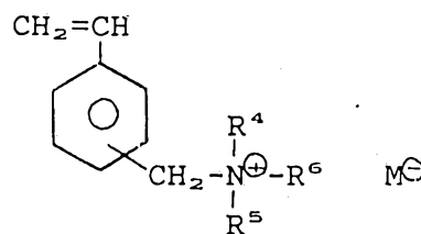
(Formula (Ib))
