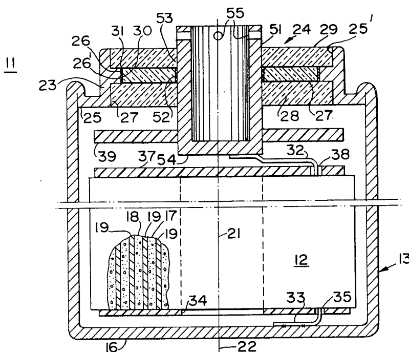
FIG. 1 (PRIOR ART)
