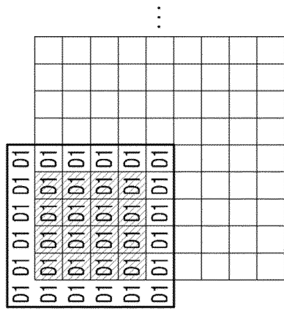
... (c) calculation of first diagonal gradient D1
