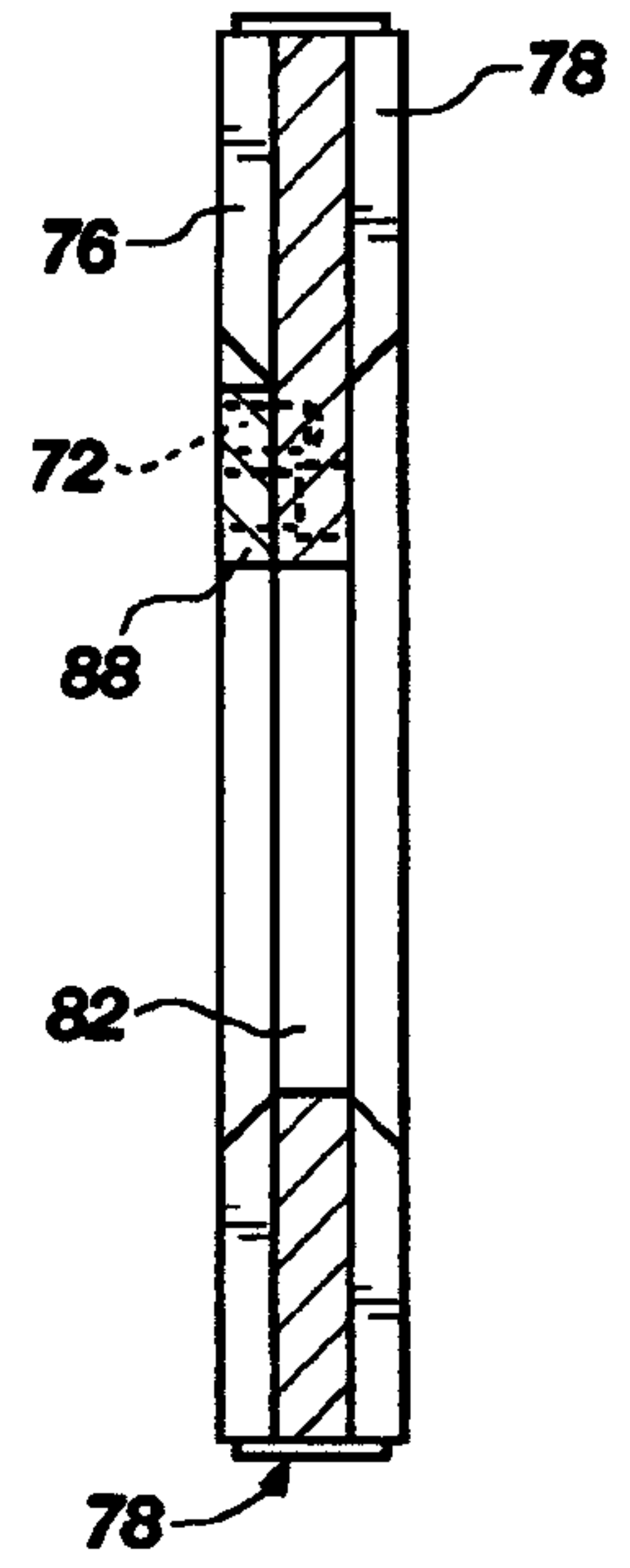
Fig. 3 (PRIOR ART)
