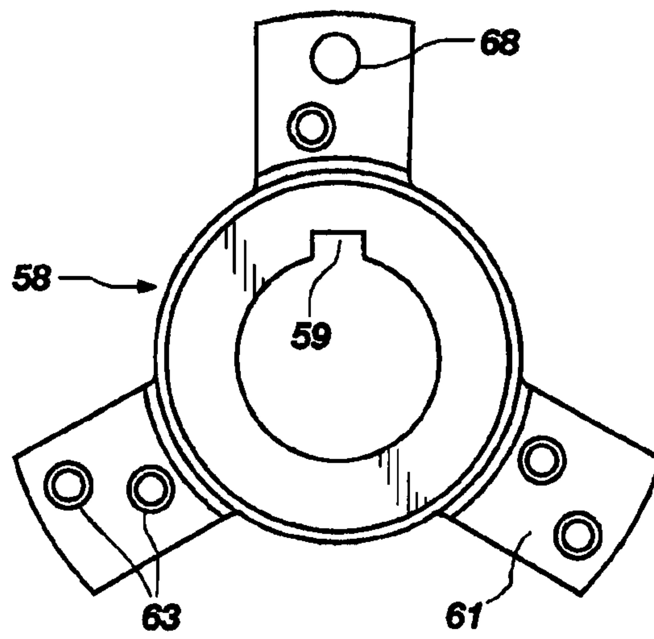
Fig. 5 (PRIOR ART)
