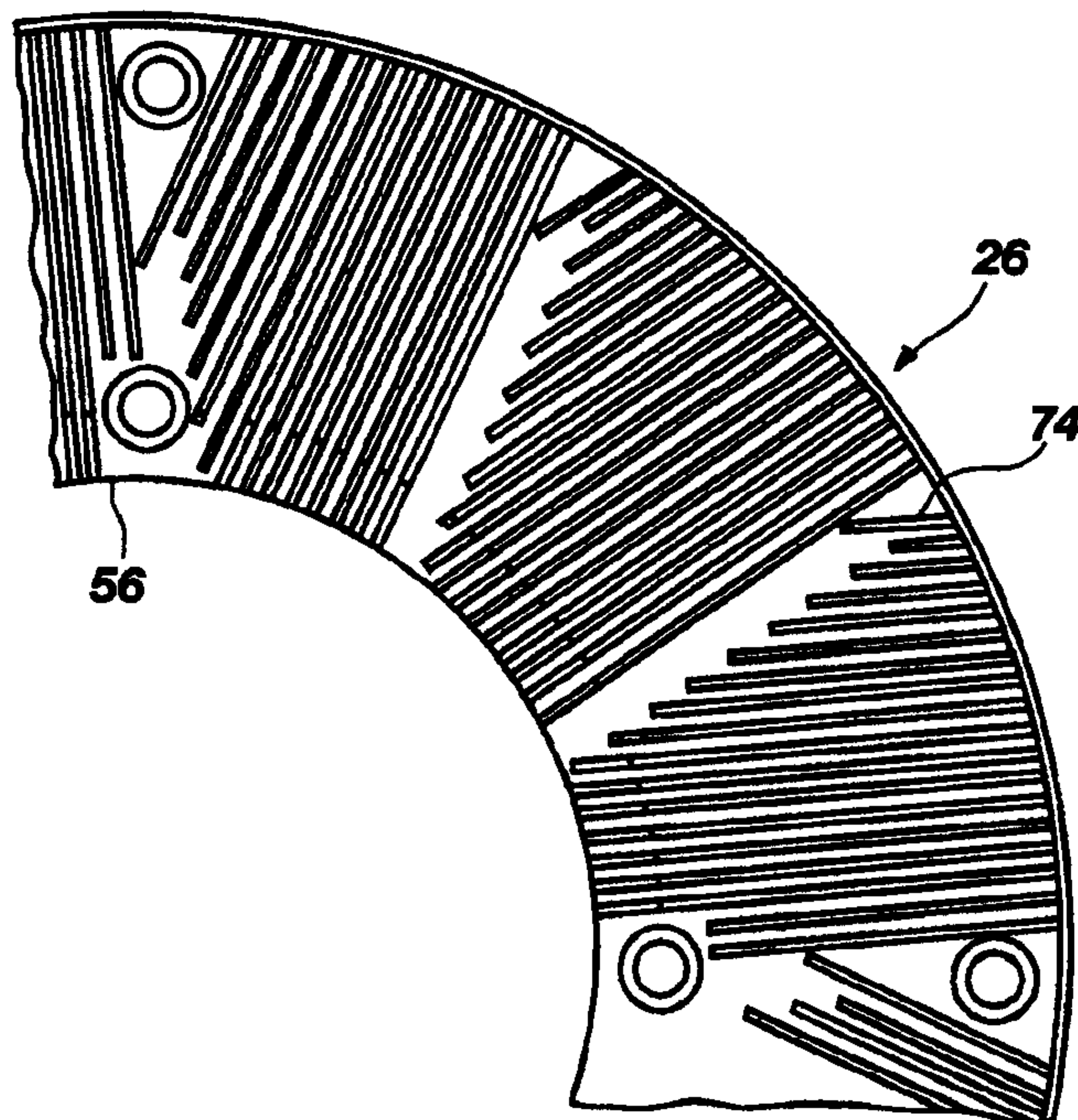
Fig. 4 (PRIOR ART)
