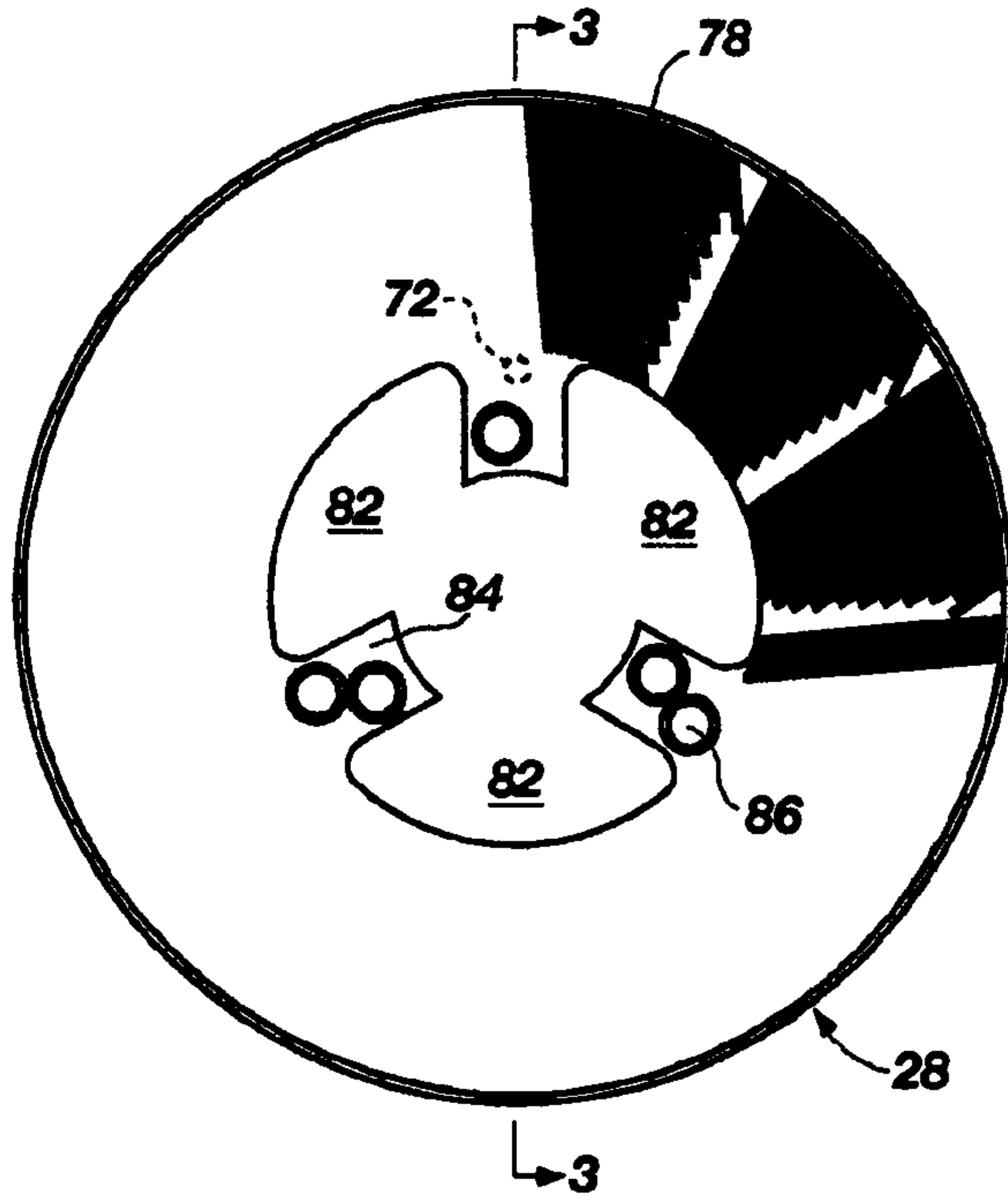
Fig. 2 (PRIOR ART)
