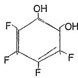
tetrachloro-o-quinol tetrafluoro-o-quinol
