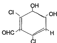
3,4-dihydroxy-2,6-dichloro-benzaldehyde
