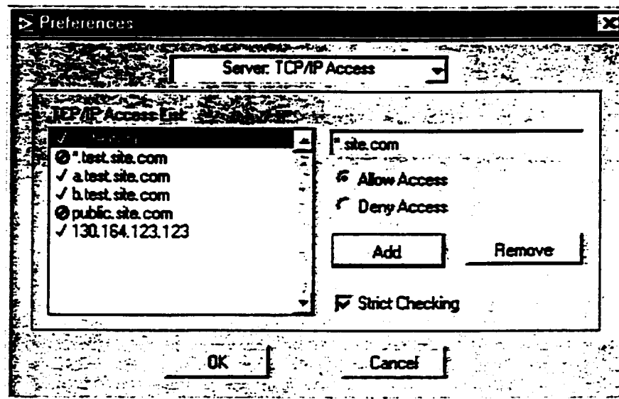
Figure 30 Server: TCP/IP Access
