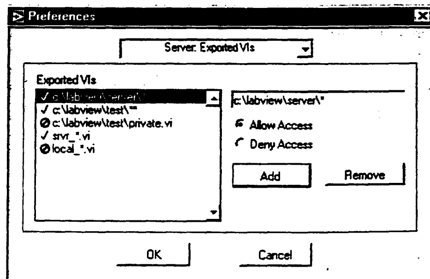
Figure 29 Server: TCP/IP Access Dialog Box
