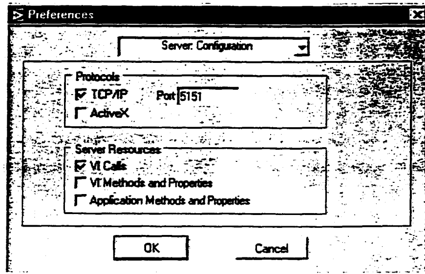
Figure 28 Server Configuration Dialog Box
