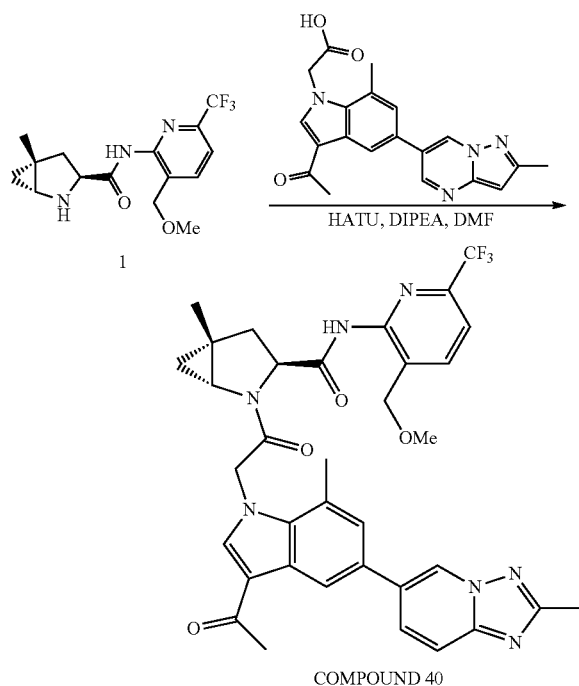
SCHEME 39. Synthesis of (1R,3S,5R)-2-(2-(3-acetyl-7-methyl-5-(2-methyl-[1,2,4]triazolo[1,5-a]pyridin-6-yl)-1H-indol-1-yl)acetyl)-N-(3-methoxymethyl)-6-(trifluoromethyl)pyridin-2-yl)-5-methyl-2-azabicyclo[3.1.0]hexane-3-carboxamide (COMPOUND 40)
