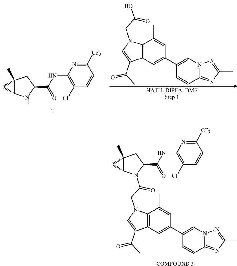
SCHEME 3: Synthesis of (1R,3S,5R)-2-(2-(3-acetyl-7-methyl-5-(2-methyl-[1,2,4]triazolo[1,5-a]pyridin-6-yl)-1H-indol-1-yl)acetyl)-N-(3-chloro-6-(trifluoromethyl)pyridin-2-yl)-5-methyl-2-azabicyclo[3.1.0]hexane-3-carboxamide (COMPOUND 3)
