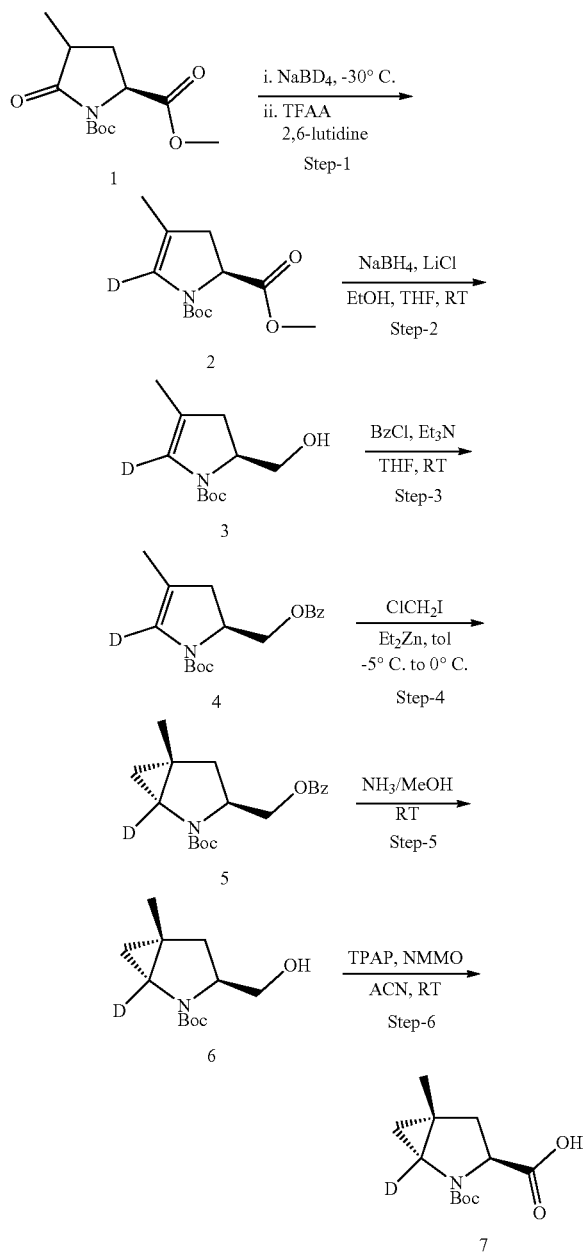
SCHEME 67. Synthesis of (1R,3S,5R)-2-(tert-butoxycarbonyl)-5-methyl-2-azabicyclo[3.1.0]hexane-3-carboxylic-1-d acid
