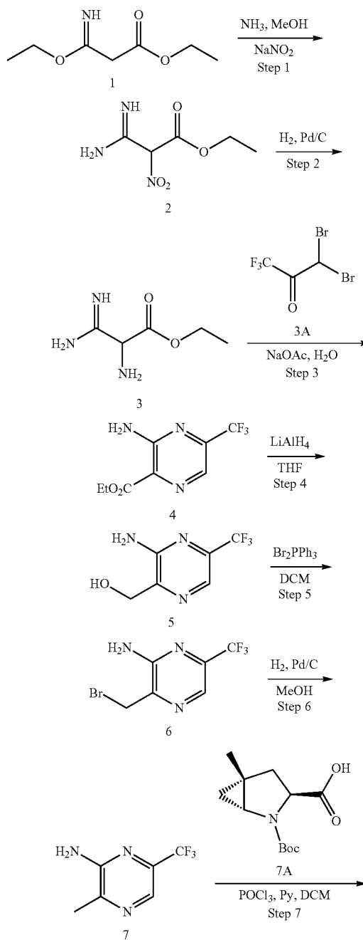
SCHEME 58. Synthesis of (1R,3S,5R)-2-(2-(3-acetyl-7-methyl-5-(2-methylpyrimidin-5-yl)-1H-indol-1-yl)acetyl)-5-methyl-N-(3-methyl-6-(trifluoromethyl)pyrazin-2-yl)-2-azabicyclo[3.1.0]hexane-3-carboxamide (COMPOUND 59)
