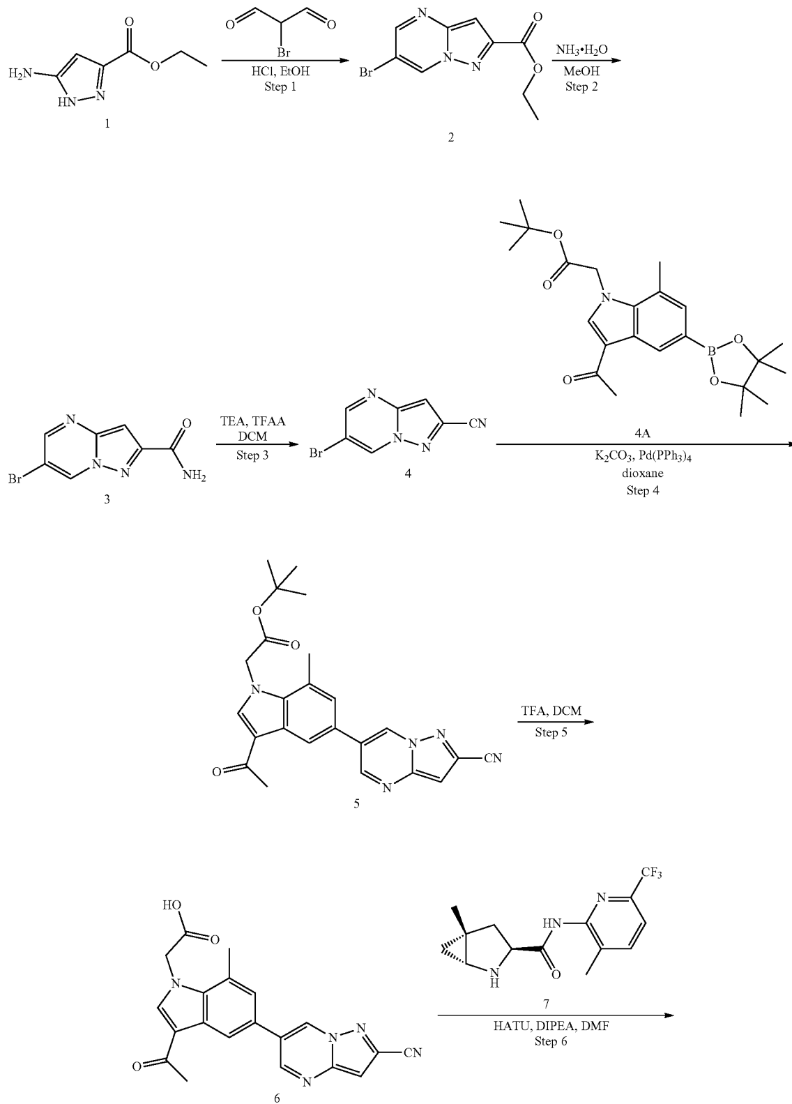
SCHEME 13. Synthesis of (1R,3S,5R)-2-(2-(3-acetyl-5-(2-cyanopyrazolo[1,5-a]pyrimidin-6-yl)-7-methyl-1H-indol-1-yl)acetyl)-5-methyl-N-(3-methyl-6-(trifluoromethyl)pyridin-2-yl)-2-azabicyclo[3.1.0]hexane-3-carboxamide (COMPOUND 13)
