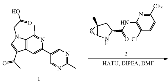
SCHEME 41. Synthesis of (1R,3S,5R)-2-(2-(3-acetyl-7-methyl-5-(2-methylpyrimidin-5-yl)-1H-pyrrolo[2,3-c]pyridin-1-yl)acetyl)-N-(3-chloro-6-(trifluoromethyl)pyridin-2-yl)-5-methyl-2-azabicyclo[3.1.0]hexane-3-carboxamide (COMPOUND 42)
