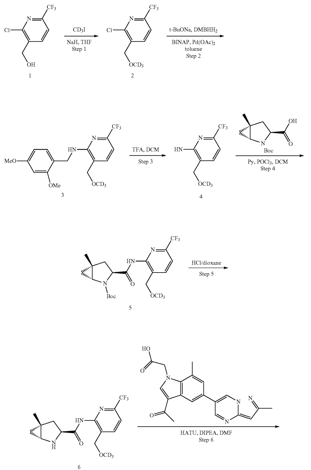
SCHEME 40. Example 2: Synthesis of (1R,3S,5R)-2-(2-(3-acetyl-7-methyl-5-(2-methylpyrazolo[1,5-a]pyrimidin-6-yl)-1H-indol-1-yl)acetyl)-N-(3-((methoxy-d 3 )methyl)-6-(trifluoromethyl)pyridin-2-yl)-5-methyl-2-azabicyclo[3.1.0]hexane-3-carboxamide (COMPOUND 80)
