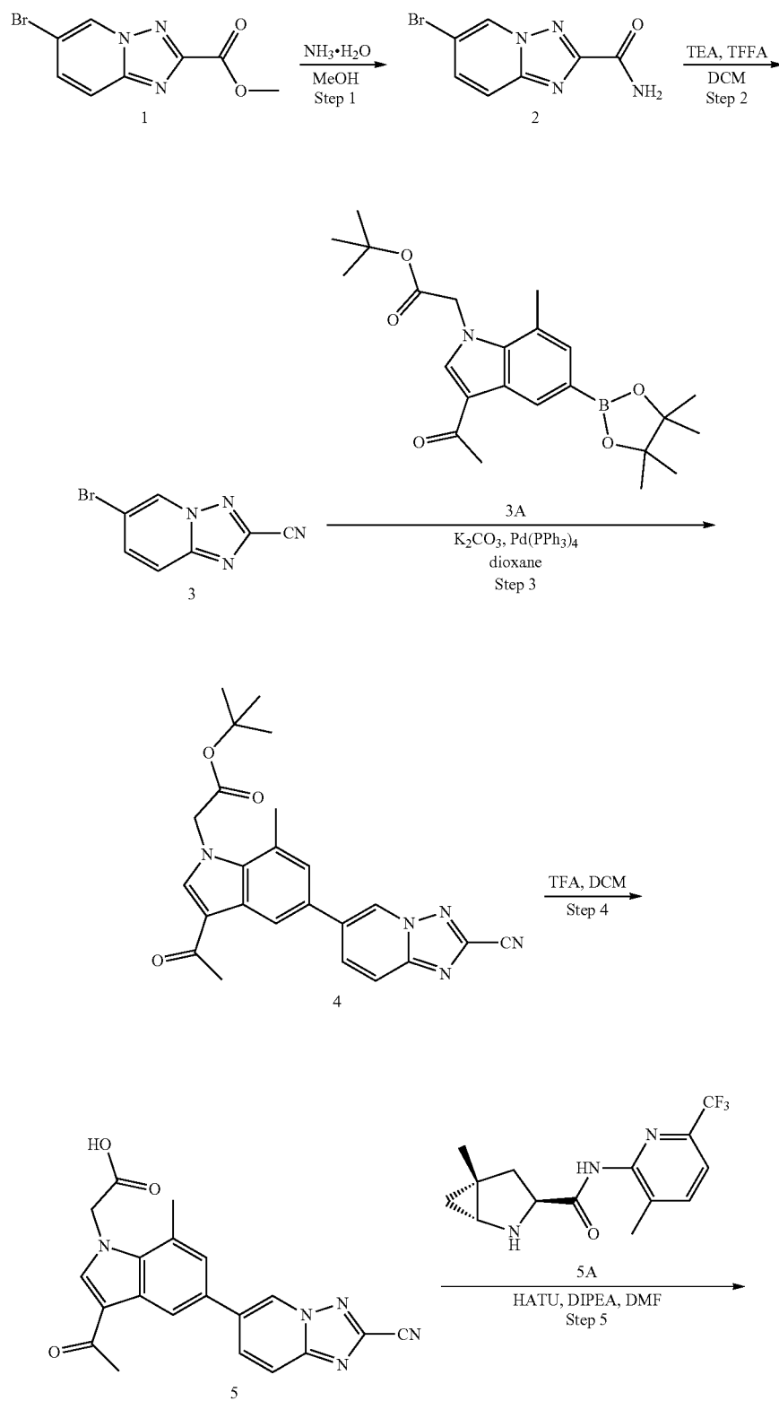
SCHEME 21. Synthesis of (1R,3S,5R)-2-(2-(3-acetyl-5-(2-cyano-[1,2,4]triazolo[1,5-a]pyridin-6-yl)-7-methyl-1H-indol-1-yl)acetyl)-5-methyl-N-(3-methyl-6-(trifluoromethyl)pyridin-2-yl)-2-azabicyclo[3.1.0]hexane-3-carboxamide (COMPOUND 22)
