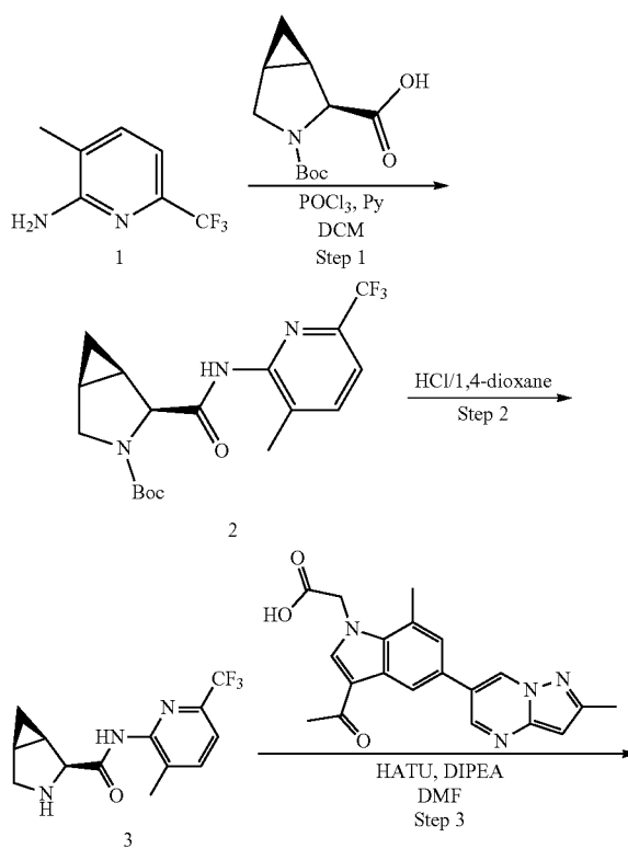
SCHEME 1. Synthesis of (1R,2S,5S)-3-(2-(3-acetyl-7-methyl-5-(2-methylpyrazolo[1,5-a]pyrimidin-6-yl)-1H-indol-1-yl)acetyl)-N-(3-methyl-6-(trifluoromethyl)pyridin-2-yl)-3-azabicyclo[3.1.0]hexane-2-carboxamide (COMPOUND 1)
