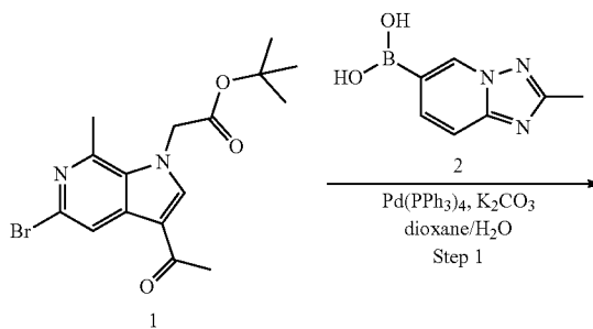
SCHEME 55. Synthesis of (1R,3S,5R)-2-(2-(3-acetyl-7-methyl-5-(2-methyl-[1,2,4]triazolo[1,5-a]pyridin-6-yl)-1H-pyrrolo[2,3-c]pyridin-1-yl)acetyl)-5-methyl-N-(3-methyl-6-(trifluoromethyl)pyridin-2-yl)-2-azabicyclo[3.1.0]hexane-3-carboxamide (COMPOUND 56)
