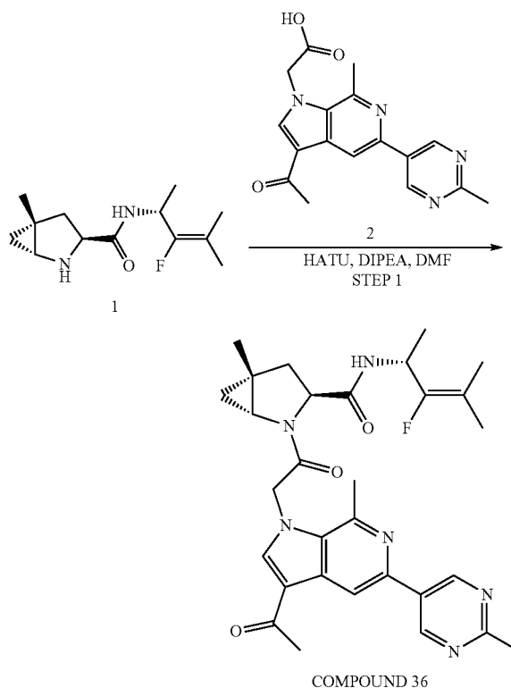
SCHEME 35. Synthesis of (1R,3S,5R)-2-(2-(3-acetyl-7-methyl-5-(2-methylpyrimidin-5-yl)-1H-pyrrolo [2,3-c]pyridin-1-yl)acetyl)-N-((R)-3-fluoro-4-methylpent-3-en-2-yl)-5-methyl-2-azabicyclo [3.1.0]hexane-3-carboxamide (COMPOUND 36)
