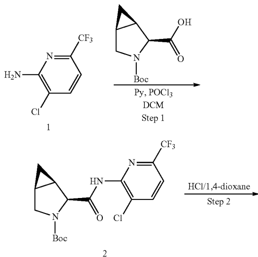
SCHEME 6: Synthesis of (1R,2S,5S)-3-(2-(3-acetyl-7-methyl-5-(2-methylpyrazolo[1,5-a]pyrimidin-6-yl)-1H-indol-1-yl)acetyl)-N-(3-chloro-6-(trifluoromethyl)pyridin-2-yl)-3-azabicyclo[3.1.0]hexane-2-carboxamide (COMPOUND 6)
