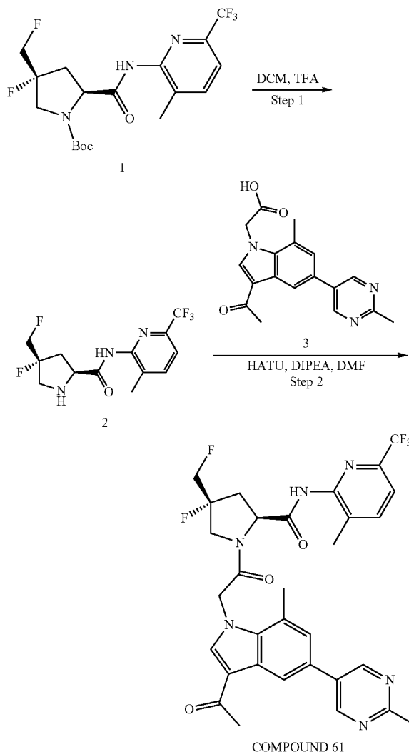
SCHEME 60. Synthesis of (2S,4R)-1-(2-(3-acetyl-7-methyl-5-(2-methylpyrimidin-5-yl)-1H-indol-1-yl)acetyl)-4-fluoro-4-(fluoromethyl)-N-(3-methyl-6-(trifluoromethyl)pyridin-2-yl)pyrrolidine-2-carboxamide (COMPOUND 61)
