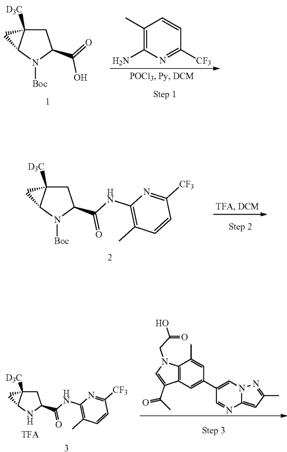
SCHEME 64 Synthesis of (1R,3S,5R)-2-(2-(3-acetyl-7-methyl-5-(2-methylpyrazolo[1,5-a]pyrimidin-6-yl)-1H-indol-1-yl)acetyl)-5-(methyl-d3)-N-(3-methyl-6-(trifluoromethyl)pyridin-2-yl)-2-azabicyclo[3.1.0]hexane-3-carboxamide (COMPOUND 75)
