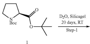
SCHEME 69. Synthesis of (1R,3S,4R,5R)-2-(2-(3-acetyl-5-(2-methylpyrimidin-5-yl)-1H-indazol-1-yl)acetyl)-N-(6-bromo-3-methylpyridin-2-yl)-5-methyl-2-azabicyclo[3.1.0]hexane-4-d-3-carboxamide (COMPOUND 78)
