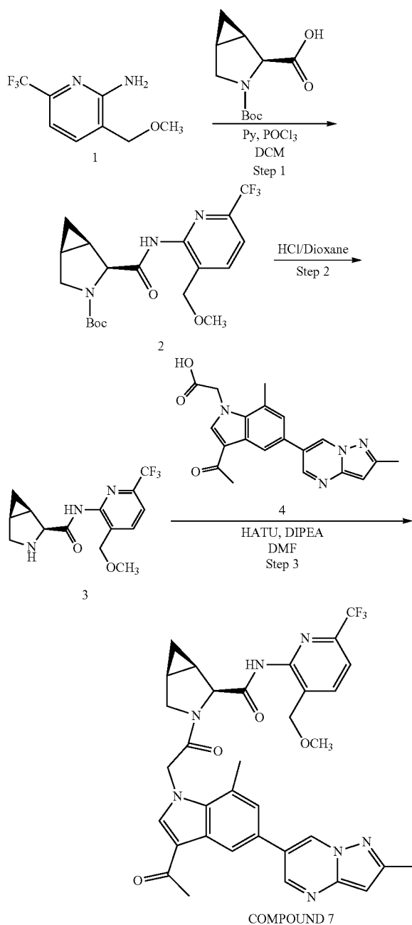
SCHEME 7: Synthesis of (1R,2S,5S)-3-(2-(3-acetyl-7-methyl-5-(2-methylpyrazolo[1,5-a]pyrimidin-6-yl)-1H-indol-1-yl)acetyl)-N-(3-(methoxymethyl)-6-(trifluoromethyl)pyridin-2-yl)-3-azabicyclo[3.1.0]hexane-2-carboxamide (COMPOUND 7)
