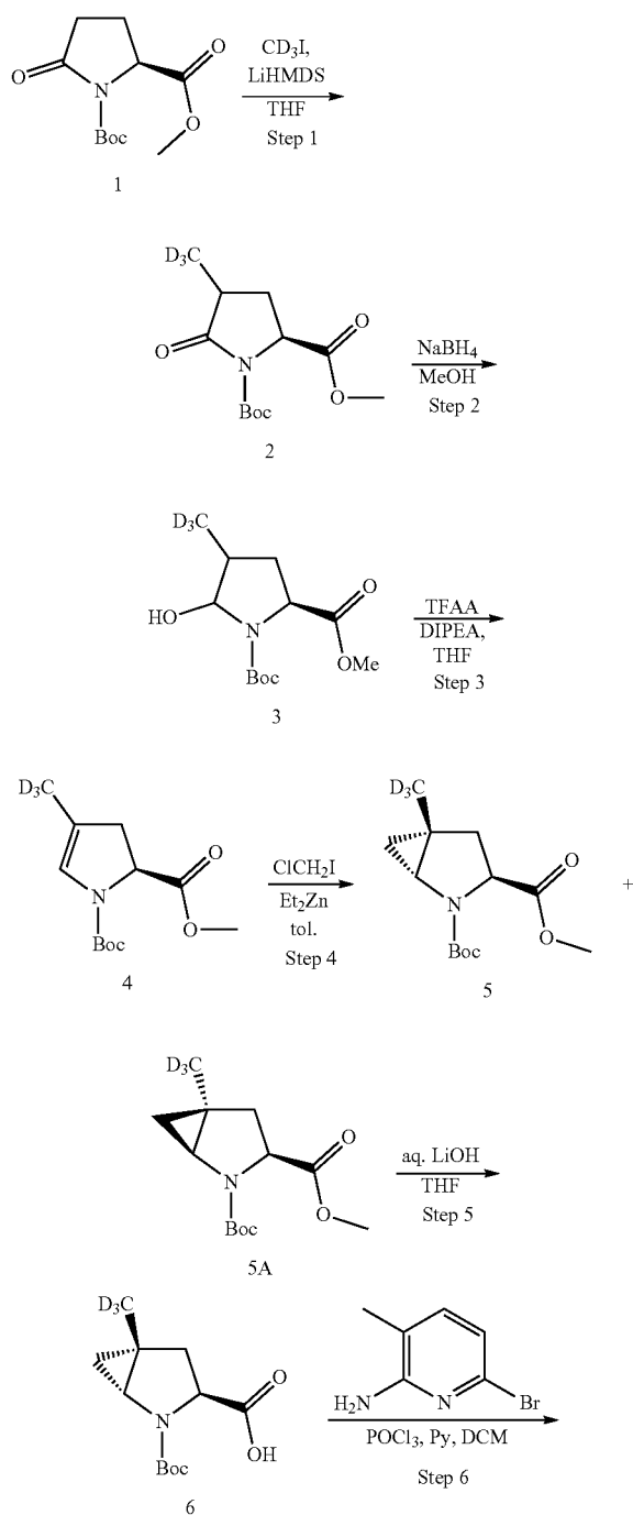
SCHEME 61. Synthesis of (1R,3S,5R)-2-(2-(3-acetyl-7-methyl-5-(2-methylpyrimidin-5-yl)-1H-indol-1-yl)acetyl)-N-(6-bromo-3-methylpyridin-2-yl)-5-(methyl-d3)-2-azabicyclo[3.1.0]hexane-3-carboxamide (COMPOUND 72)
