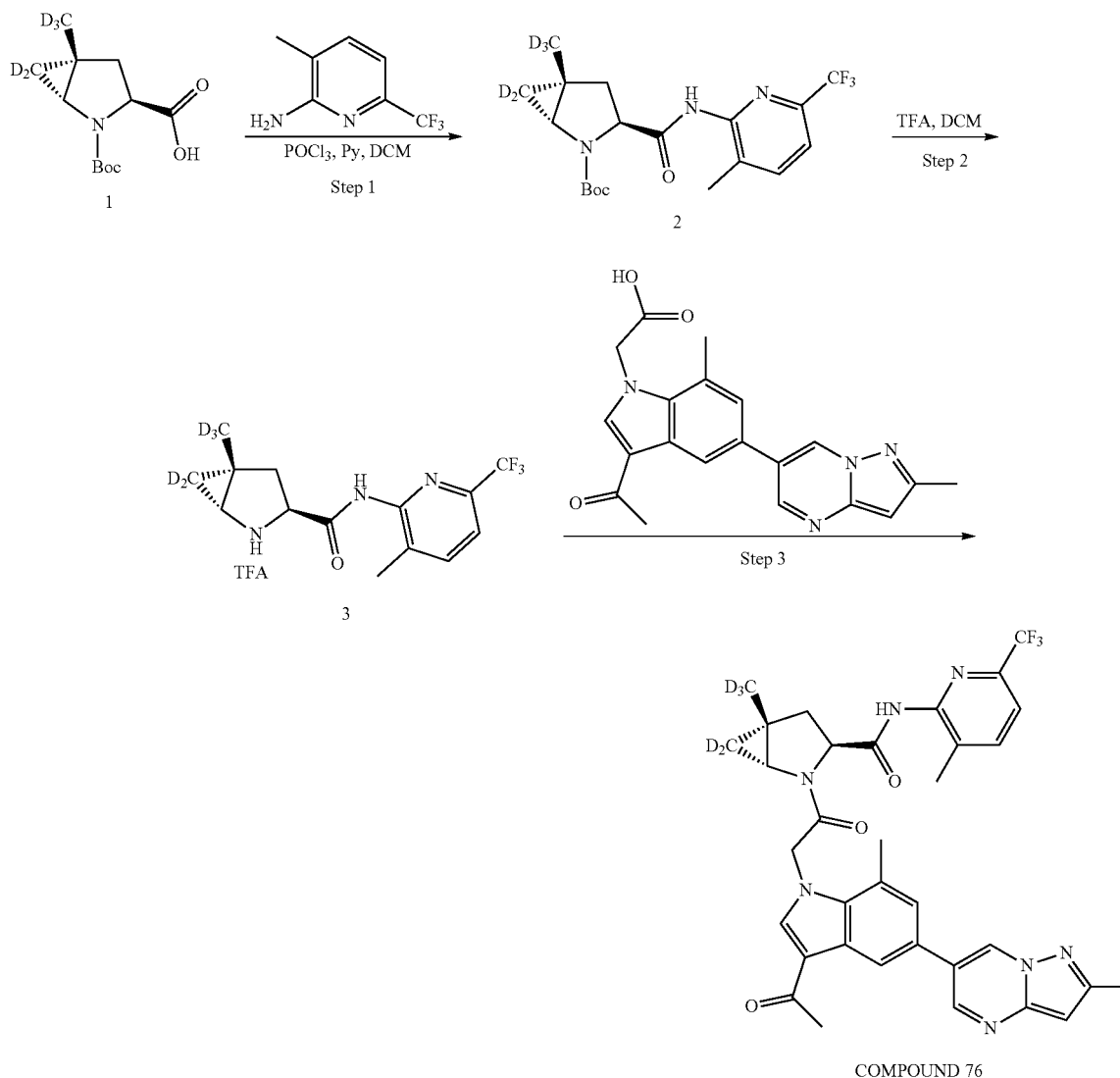
SCHEME 65. Synthesis of (1R,3S,5R)-2-(2-(3-acetyl-7-methyl-5-(2-methylpyrazolo[1,5-a]pyrimidin-6-yl)-1H-indol-1-yl)acetyl)-5-(methyl-d3)-N-(3-methyl-6-(trifluoromethyl)pyridin-2-yl)-2-azabicyclo[3.1.0]hexane-6,6-d2-3-carboxamide (COMPOUND 76)
