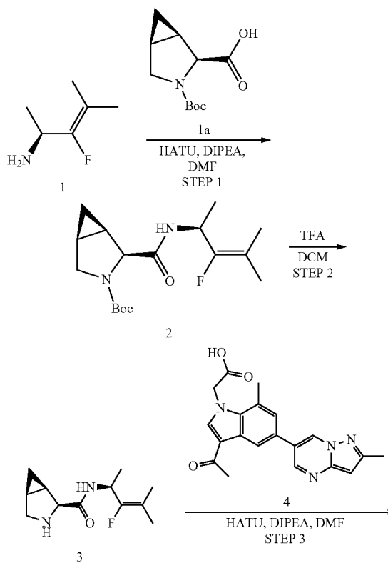
SCHEME 37. Synthesis of (1R,2S,5S)-3-(2-(3-acetyl-7-methyl-5-(2-methylpyrazolo[1,5-a]pyrimidin-6-yl)-1H-indol-1-yl)acetyl)-N-((S)-3-fluoro-4-methylpent-3-en-2-yl)-3-azabicyclo[3.1.0]hexane-2-carboxamide (COMPOUND 38)
