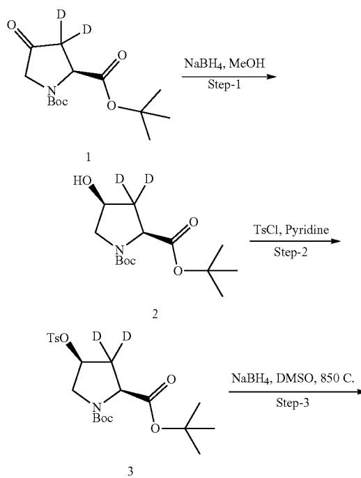
SCHEME 70. Synthesis of (1R,3S,5R)-2-(2-(3-acetyl-5-(2-methylpyrimidin-5-yl)-1H-indazol-1-yl)acetyl)-N-(6-bromo-3-methylpyridin-2-yl)-5-methyl-2-azabicyclo[3.1.0]hexane-4,4-d 2 -3-carboxamide (COMPOUND 79)
