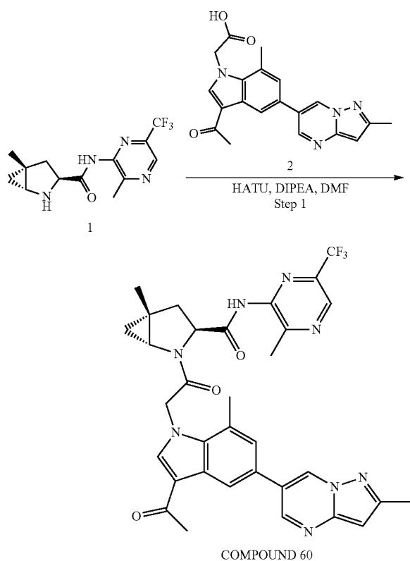
SCHEME 59. Synthesis of (1R,3S,5R)-2-(2-(3-acetyl-7-methyl-5-(2-methylpyrazolo[1,5-a]pyrimidin-6-yl)-1H-indol-1-yl)acetyl)-5-methyl-N-(3-methyl-6-(trifluoromethyl)pyridin-2-yl)-2-azabicyclo[3.1.0]hexane-3-carboxamide (COMPOUND 60)
