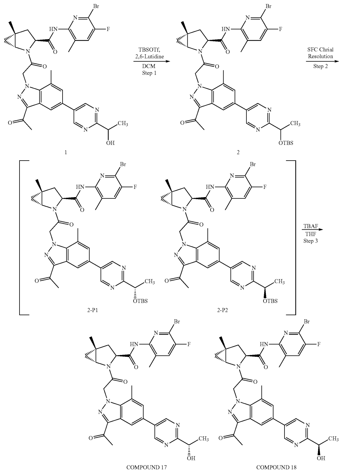
SCHEME 17. Synthesis of (1R,3S,5R)-2-(2-(3-acetyl-5-(2-((S)-1-hydroxyethyl)pyrimidin-5-yl)-7-methyl-1H-indazol-1-yl)acetyl)-N-(6-bromo-5-fluoro-3-methylpyridin-2-yl)-5-methyl-2-azabicyclo[3.1.0]hexane-3-carboxamide (COMPOUND 17) and (1R,3S,5R)-2-(3-acetyl-5-(2-((R)-1-hydroxyethyl)pyrimidin-5-yl)-7-methyl-1H-indazol-1-yl)acetyl)-N-(6-bromo-5-fluoro-3-methylpyridin-2-yl)-5-methyl-2-azabicyclo[3.1.0]hexane-3-carboxamide (COMPOUND 18)
