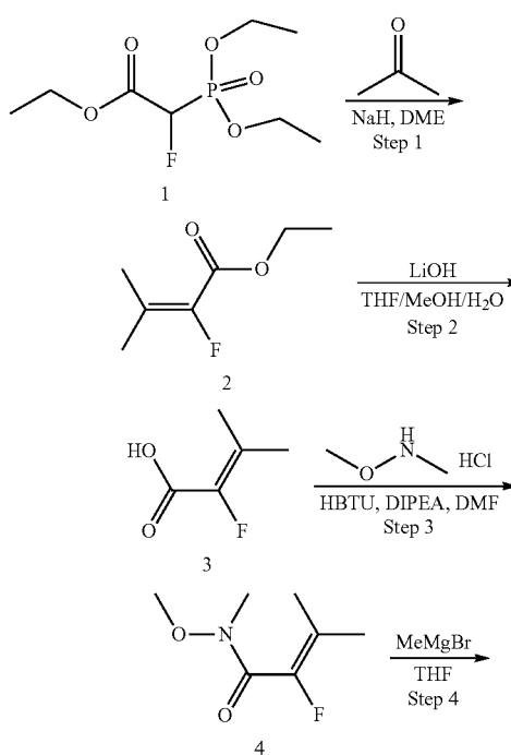
SCHEME 26. Synthesis of (1R,3S,5R)-2-(2-(3-acetyl-7-methyl-5-(2-methylpyrazolo[1,5-a]pyrimidin-6-yl)-1H-indol-1-yl)acetyl)-N-((R)-3-fluoro-4-methylpent-3-en-2-yl)-5-methyl-2-azabicyclo[3.1.0]hexane-3-carboxamide (COMPOUND 27)
