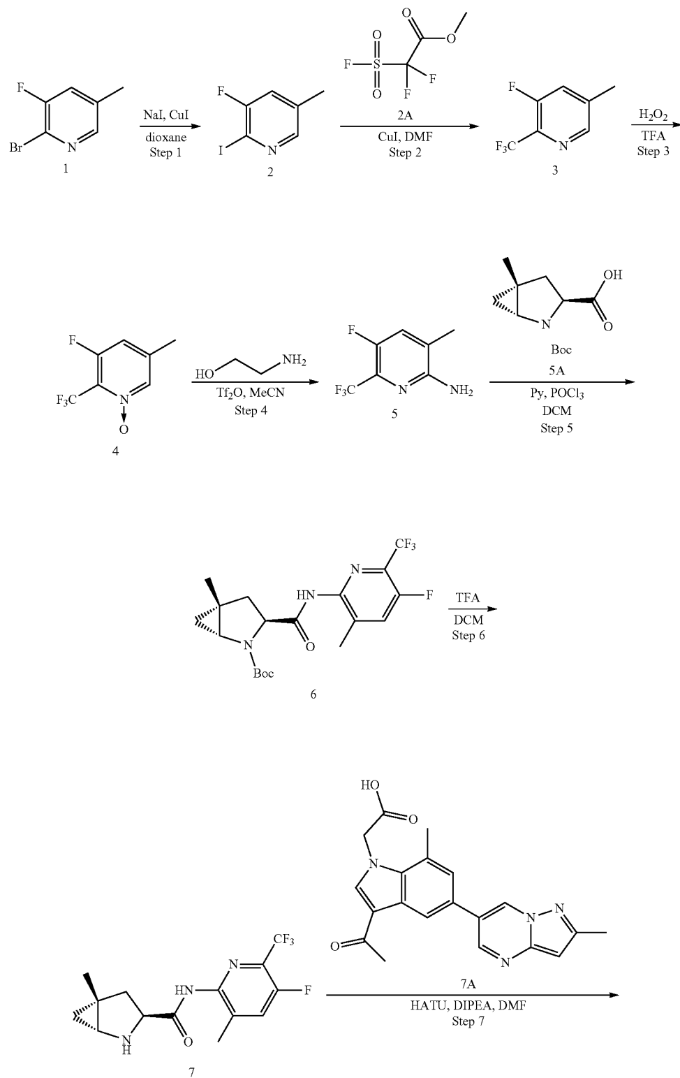
SCHEME 16. (1R,3S,5R)-2-(2-(3-acetyl-7-methyl-5-(2-methylpyrazolo[1,5-a]pyrimidin-6-yl)-1H-indol-1-yl)acetyl)-N-(5-fluoro-3-methyl-6-(trifluoromethyl)pyridin-2-yl)-5-methyl-2-azabicyclo[3.1.0]hexane-3-carboxamide (COMPOUND 16)
