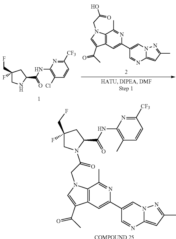
SCHEME 24. Synthesis of (2S,4R)-1-(2-(3-acetyl-7-methyl-5-(2-methylpyrazolo[1,5-a]pyrimidin-6-yl)-1H-pyrrolo[2,3-c]pyridin-1-yl)acetyl)-4-fluoro-4-(fluoromethyl)-N-(3-methyl-6-(trifluoromethyl)pyridin-2-yl)pyrrolidine-2-carboxamide (COMPOUND 25)
