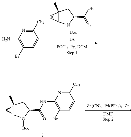
SCHEME 22. Synthesis of (1R,3S,5R)-2-(2-(3-acetyl-7-methyl-5-(2-methylpyrazolo[1,5-a]pyrimidin-6-yl)-1H-pyrrolo[2,3-c]pyridin-1-yl)acetyl)-N-(3-cyano-6-(trifluoromethyl)pyridin-2-yl)-5-methyl-2-azabicyclo[3.1.0]hexane-3-carboxamide (COMPOUND 23)
