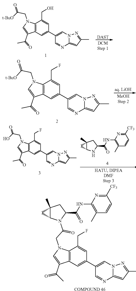
SCHEME 45. Synthesis of (1R,3S,5R)-2-(2-(3-acetyl-7-(fluoromethyl)-5-(2-methylpyrazolo[1,5-a]pyrimidin-6-yl)-1H-indol-1-yl)acetyl)-5-methyl-N-(3-methyl-6-(trifluoromethyl)pyridin-2-yl)-2-azabicyclo[3.1.0]hexane-3-carboxamide (COMPOUND 46)
