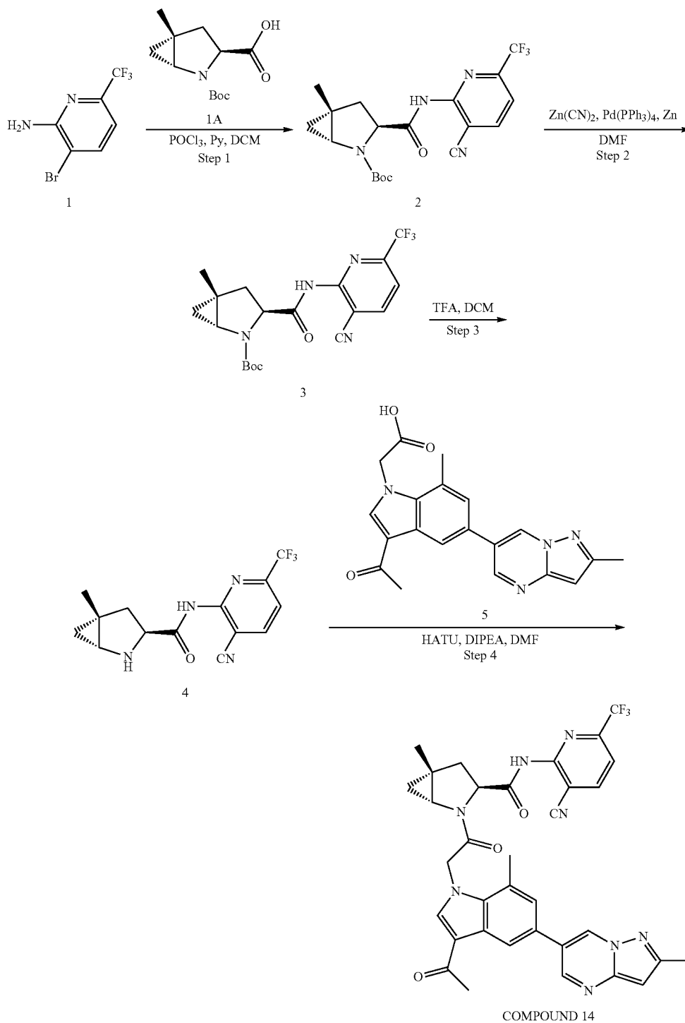
SCHEME 14. Synthesis of (1R,3S,5R)-2-(2-(3-acetyl-7-methyl-5-(2-methylpyrazolo[1,5-a]pyrimidin-6-yl)-1H-indol-1-yl)acetyl)-N-(3-cyano-6-(trifluoromethyl)pyridin-2-yl)-5-methyl-2-azbicyclo[3.1.0]hexane-3-carboxamide (COMPOUND 14)
