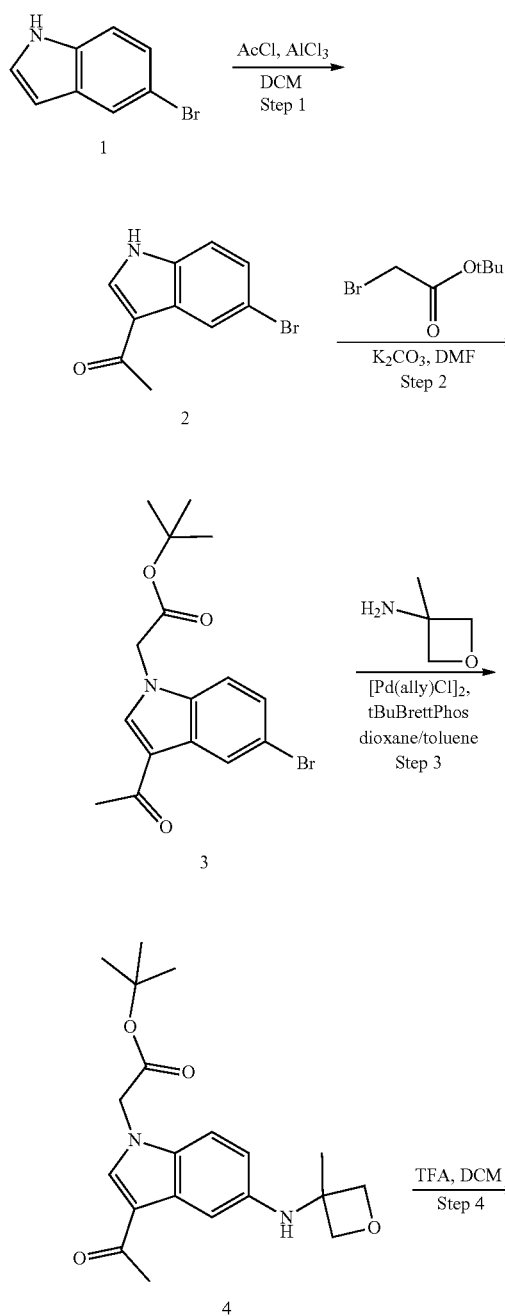
SCHEME 25. Synthesis of (1R,3S,5R)-2-(2-(3-acetyl-5-((3-methyloxetan-3-yl)amino)-1H-indol-1-yl)acetyl)-N-(6-bromo-3-methylpyridin-2-yl)-5-methyl-2-azabicyclo[3.1.0]hexane-3-carboxamide (COMPOUND 26)
