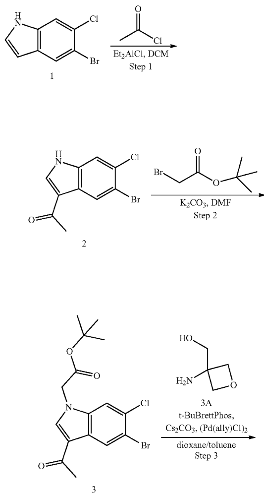
SCHEME 19. Synthesis of (1R,3S,5R)-2-(2-(8'-acetyl-3'H-spiro[oxetane-3,2'-[1,4]oxazino[3,2-f]indol]-6'(1'H)-yl)acetyl)-N-(6-bromo-3-methylpyridin-2-yl)-5-methyl-2-azabicyclo[3.1.0]hexane-3-carboxamide (COMPOUND 20)
