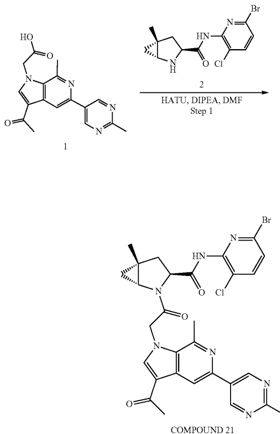
SCHEME 20. Synthesis of (1R,3S,5R)-2-(2-(3-acetyl-7-methyl-5-(2-methylpyrimidin-5-yl)-1H-pyrrolo[2,3-c]pyridin-1-yl)acetyl)-N-(6-bromo-3-chloropyridin-2-yl)-5-methyl-2-azabicyclo[3.1.0]hexane-3-carboxamide (COMPOUND 21)
