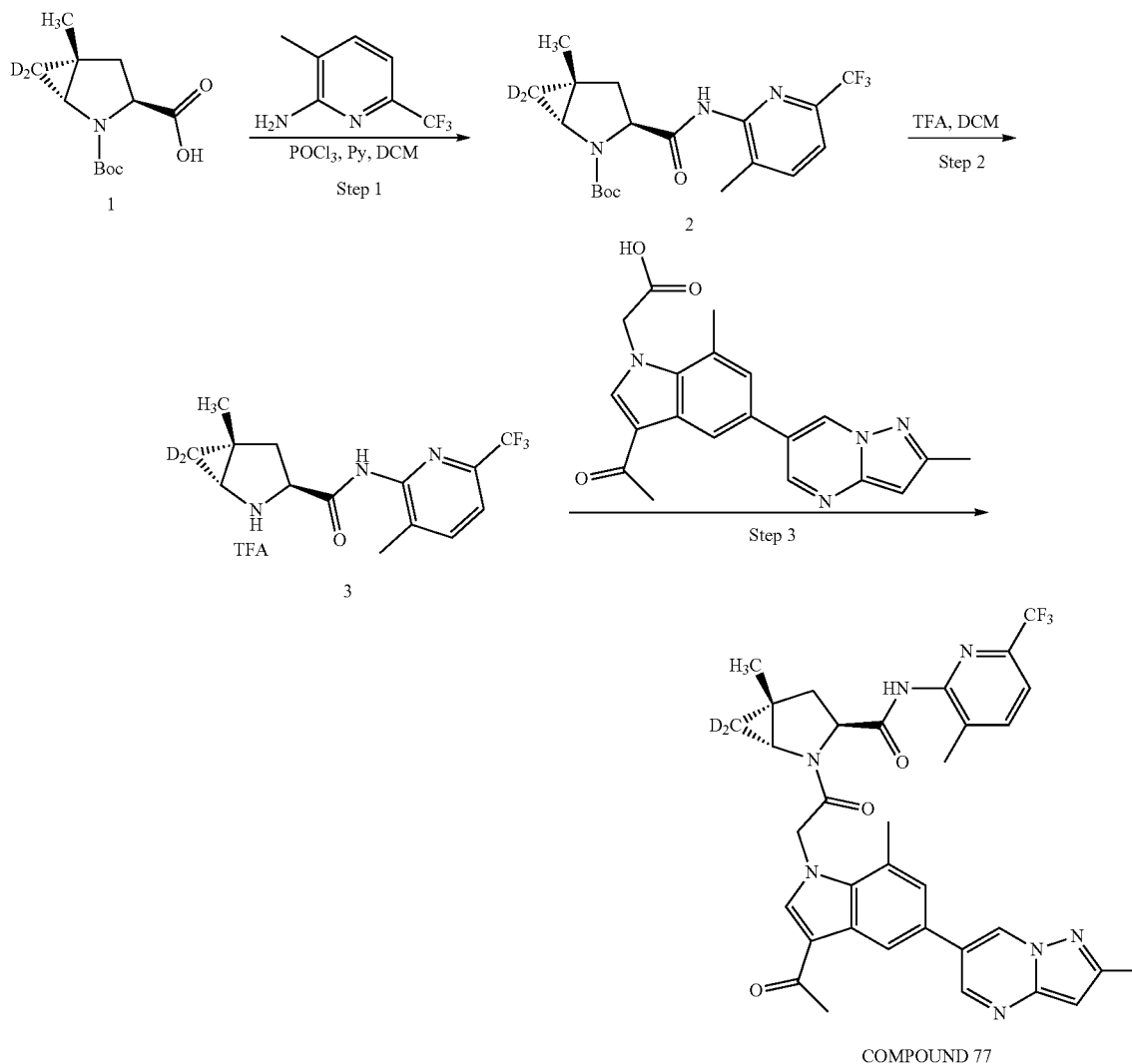
SCHEME 66. Synthesis of (1R,3S,5R)-2-(2-(3-acetyl-7-methyl-5-(2-methylpyrazolo[1,5-a]pyrimidin-6-yl)-1H-indol-1-yl)acetyl)-5-methyl-N-(3-methyl-6-(trifluoromethyl)pyridin-2-yl)-2-azabicyclo[3.1.0]hexane-6,6-d2-3-carboxamide (COMPOUND 77)
