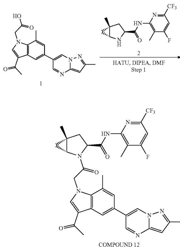
SCHEME 12. Synthesis of (1R,3S,5R)-2-(2-(3-acetyl-7-methyl-5-(2-methylpyrazolo[1,5-a]pyrimidin-6-yl)-1H-indol-1-yl)acetyl)-N-(4-fluoro-3-methyl-6-trifluoromethyl)pyridin-2-yl)-5-methyl-2-azabicyclo[3.1.0]hexane-3-carboxamide (COMPOUND 12)
