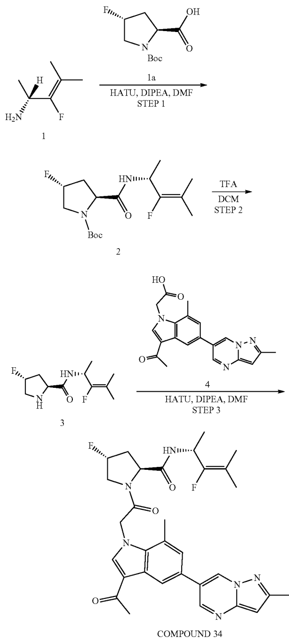
SCHEME 33. Synthesis of (2S,4R)-1-(2-(3-acetyl-7-methyl-5-(2-methylpyrazolo[1,5-a]pyrimidin-6-yl)-1H-indol-1-yl)acetyl)-4-fluoro-N-((R)-3-fluoro-4-methylpent-3-en-2-yl)pyrrolidine-2-carboxamide (COMPOUND 34)
