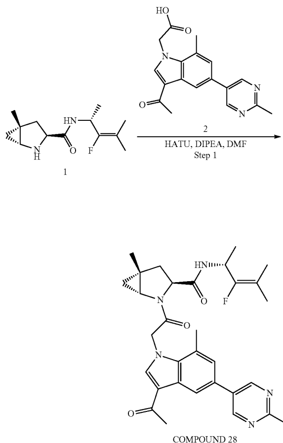
SCHEME 27. Synthesis of (1R,3S,5R)-2-(2-(3-acetyl-7-methyl-5-(2-methylpyrimidin-5-yl)-1H-indol-1-yl)acetyl)-N-((R)-3-fluoro-4-methylpent-3-en-2-yl)-5-methyl-2-azabicyclo[3.1.0]hexane-3-carboxamide (COMPOUND 28)
