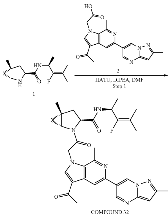
SCHEME 31. Synthesis of (1R,3S,5R)-2-(2-(3-acetyl-7-methyl-5-(2-methylpyrazolo[1,5-a]pyrimidin-6-yl)-1H-pyrrolo[2,3-c]pyridin-1-yl)acetyl)-N-((S)-3-fluoro-4-methylpent-3-en-2-yl)-5-methyl-2-azabicyclo[3.1.0]hexane-3-carboxamide (COMPOUND 32)
