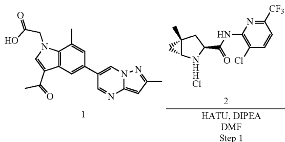
SCHEME 50. Synthesis of (1R,3S,5R)-2-(2-(3-acetyl-7-methyl-5-(2-methylpyrazolo[1,5-a]pyrimidin-6-yl)-1H-indol-1-yl)acetyl)-N-(3-chloro-6-(trifluoromethyl)pyridin-2-yl)-5-methyl-2-azabicyclo[3.1.0]hexane-3-carboxamide (COMPOUND 51)
