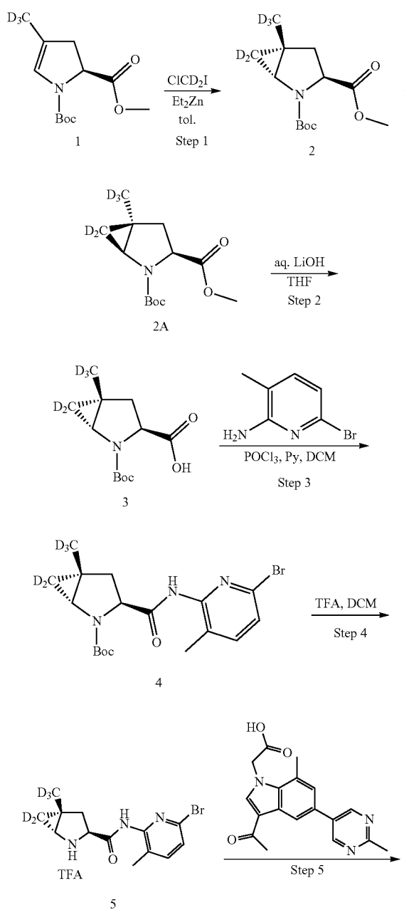
SCHEME 62. Synthesis of (1R,3S,5R)-2-(2-(3-acetyl-7-methyl-5-(2-methylpyrimidin-5-yl)-1H-indol-1-yl)acetyl)-N-(6-bromo-3-methylpyridin-2-yl)-5-(methyl-d3)-2-azabicyclo[3.1.0]hexane-6,6-d2-3-carboxamide (COMPOUND 73)
