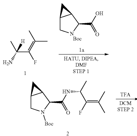
SCHEME 34. Synthesis of (1R,2S,5S)-3-(2-(3-acetyl-7-methyl-5-(2-methylpyrazolo[1,5-a]pyrimidin-6-yl)-1H-indol-1-yl)acetyl)-N-((R)-3-fluoro-4-methylpent-3-en-2-yl)-3-azabicyclo[3.1.0]hexane-2-carboxamide (COMPOUND 35)
