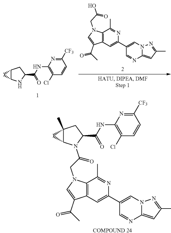
SCHEME 23. Synthesis of (1R,3S,5R)-2-(2-(3-acetyl-7-methyl-5-(2-methylpyrazolo[1,5-a]pyrimidin-6-yl)-1H-pyrrolo[2,3-c]pyridin-1-yl)acetyl)-N-(3-chloro-6-(trifluoromethyl)pyridin-2-yl)-5-methyl-2-azabicyclo[3.1.0]hexane-3-carboxamide (COMPOUND 24)
