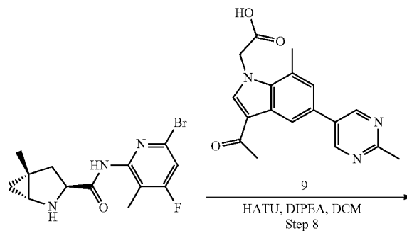
SCHEME 15. Synthesis of (1R,3S,5R)-2-(2-(3-acetyl-7-methyl-5-(2-methylpyrimidin-5-yl)-1H-indol-1-yl)acetyl)-N-(6-bromo-4-fluoro-3-methylpyridin-2-yl)-5-methyl-2-azabicyclo[3.1.0]hexane-3-carboxamide (COMPOUND 15)
