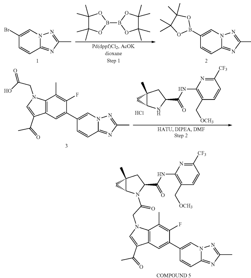
SCHEME 5: Synthesis of (1R,3S,5R)-2-(3-acetyl-6-fluoro-7-methyl-5-(2-methyl-[1,2,4]triazol[1,5-a]pyridin-6-yl)-1H-indol-1-yl)acetyl)-N-(3-(methoxymethyl)-6-(trifluoromethyl)pyridin-2-yl)-5-methyl-2-azabicyclo[3.1.0]hexane-3-carboxamide
