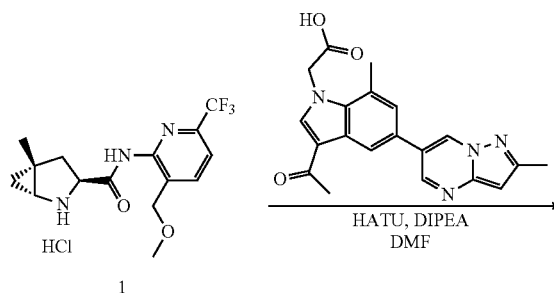
SCHEME 52. Synthesis of: (1R,3S,5R)-2-(2-(3-acetyl-7-methyl-5-(2-methylpyrazolo[1,5-a]pyrimidin-6-yl)-1H-indol-1-yl)acetyl)-N-(3-(methoxymethyl)-6-(trifluoromethyl)pyridin-2-yl)-5-methyl-2-azabicyclo[3.1.0]hexane-3-carboxamide (COMPOUND 53)
