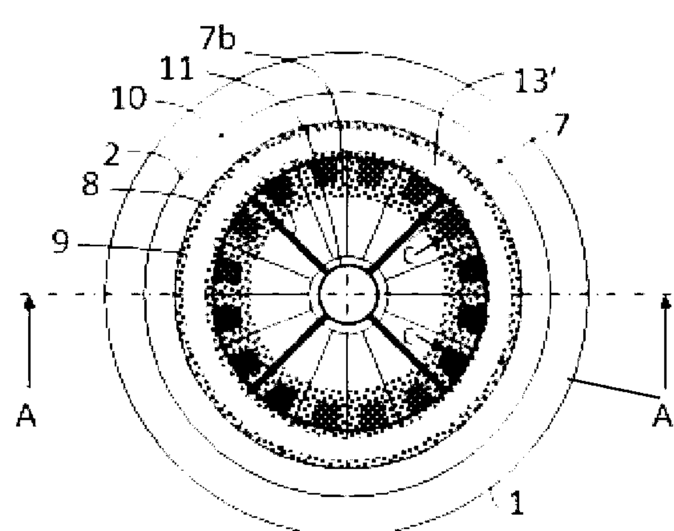
a) Top View
