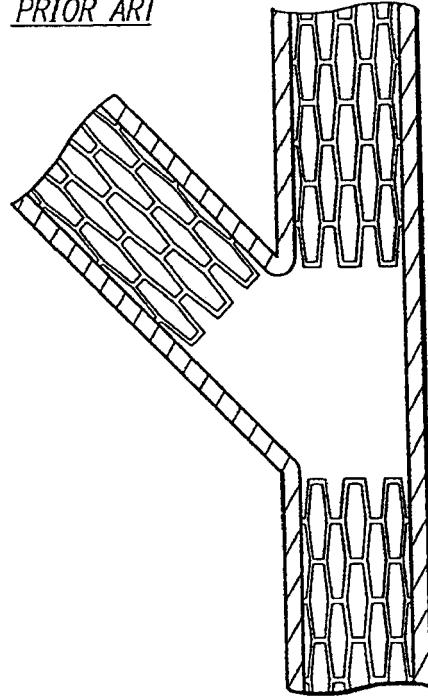
FIG. 2 PRIOR ART
