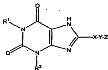
Formula I where R³ is hydrogen
