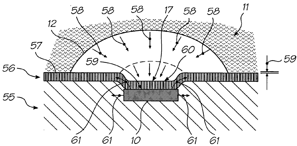
FIG. 47 (PRIOR ART)
