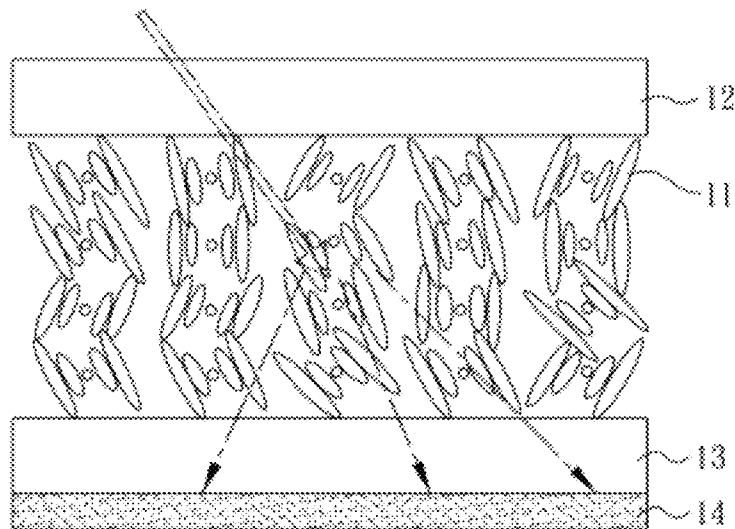
FIG. 3(Prior Art)
