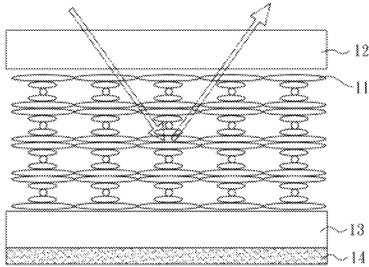
FIG. 2(Prior Art)
