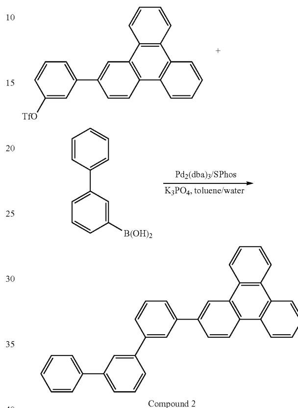
Synthesis of Single Triphenylene Compound 3
