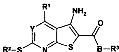
Formula II
