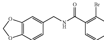
Compound 3:
