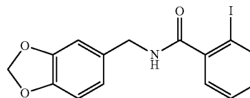
Compound 4:
