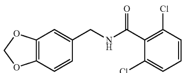
Compound 1: (N-(1,3-benzodioxol-5-ylmethyl)-2,6-dichlorobenzamide)
