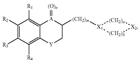
Formula VIIa
