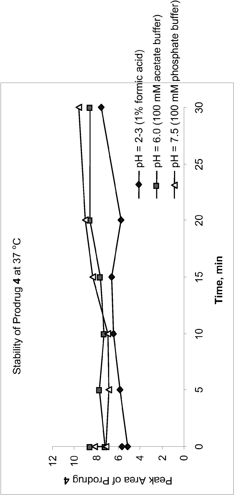
FIG. 8 Chemical Stability of Prodrug 4
