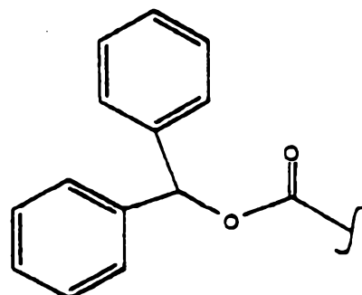
f. Structure of Bhoc Group.
