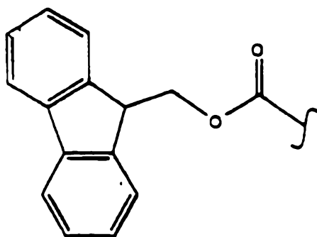
e. Structure of Fmoc Group.
