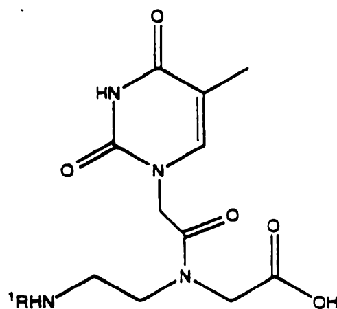
d. Structure of Fmoc-T-OH.
