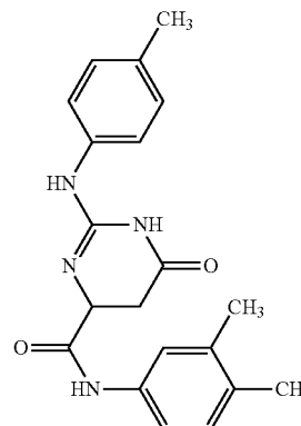
N-(3,4-dimethylphenyl)-2-((4-methylphenyl)amino)-6-oxo-1,4,5,6-tetrahydro-4-pyrimidinecarboxamide
