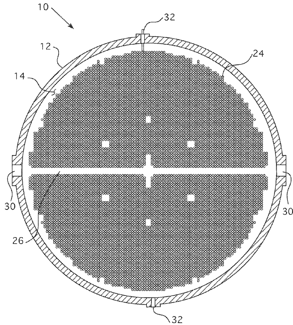
FIG. 2 Prior Art
