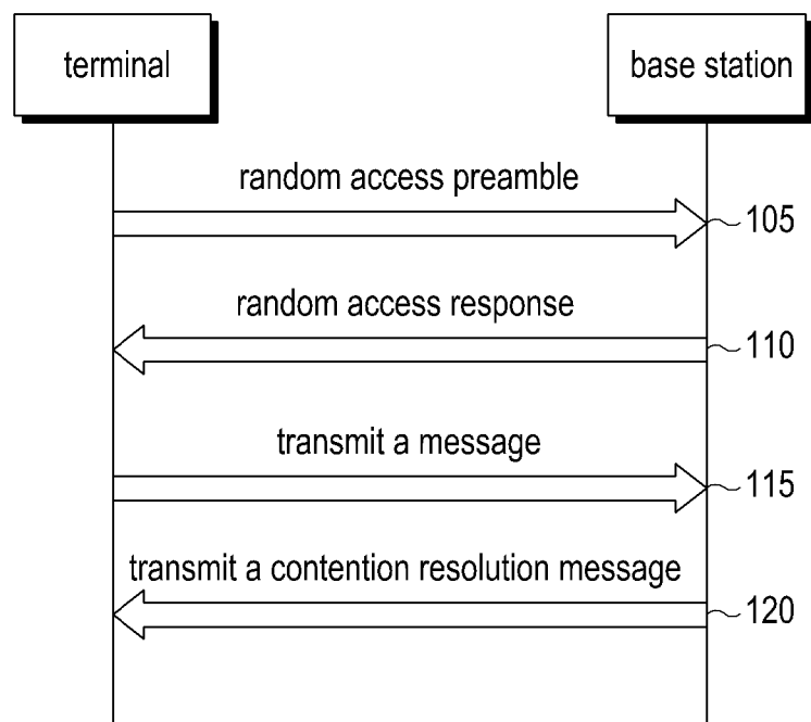
FIG.1 (RELATED ART)
