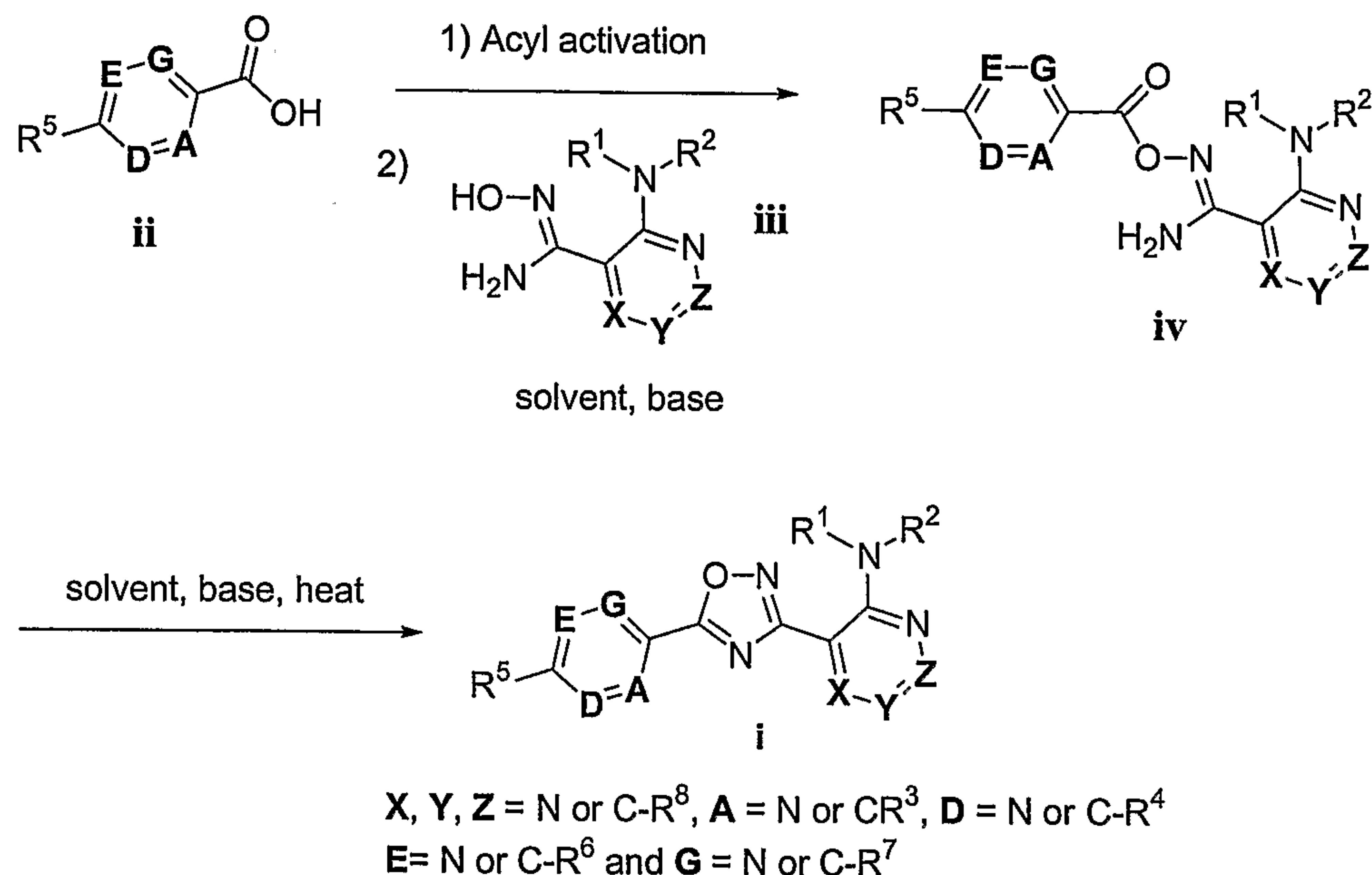
Scheme 1
