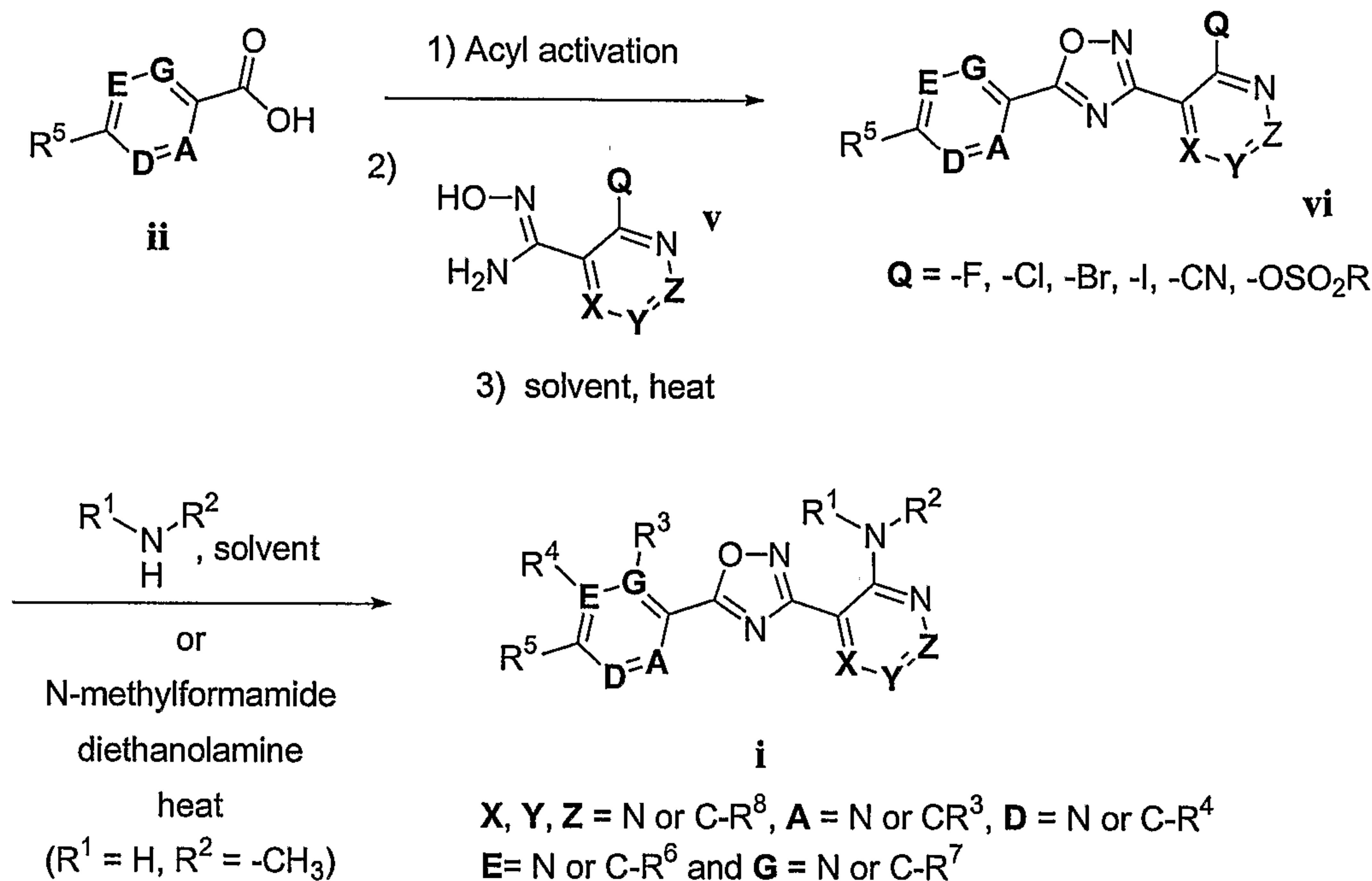
Scheme 2
