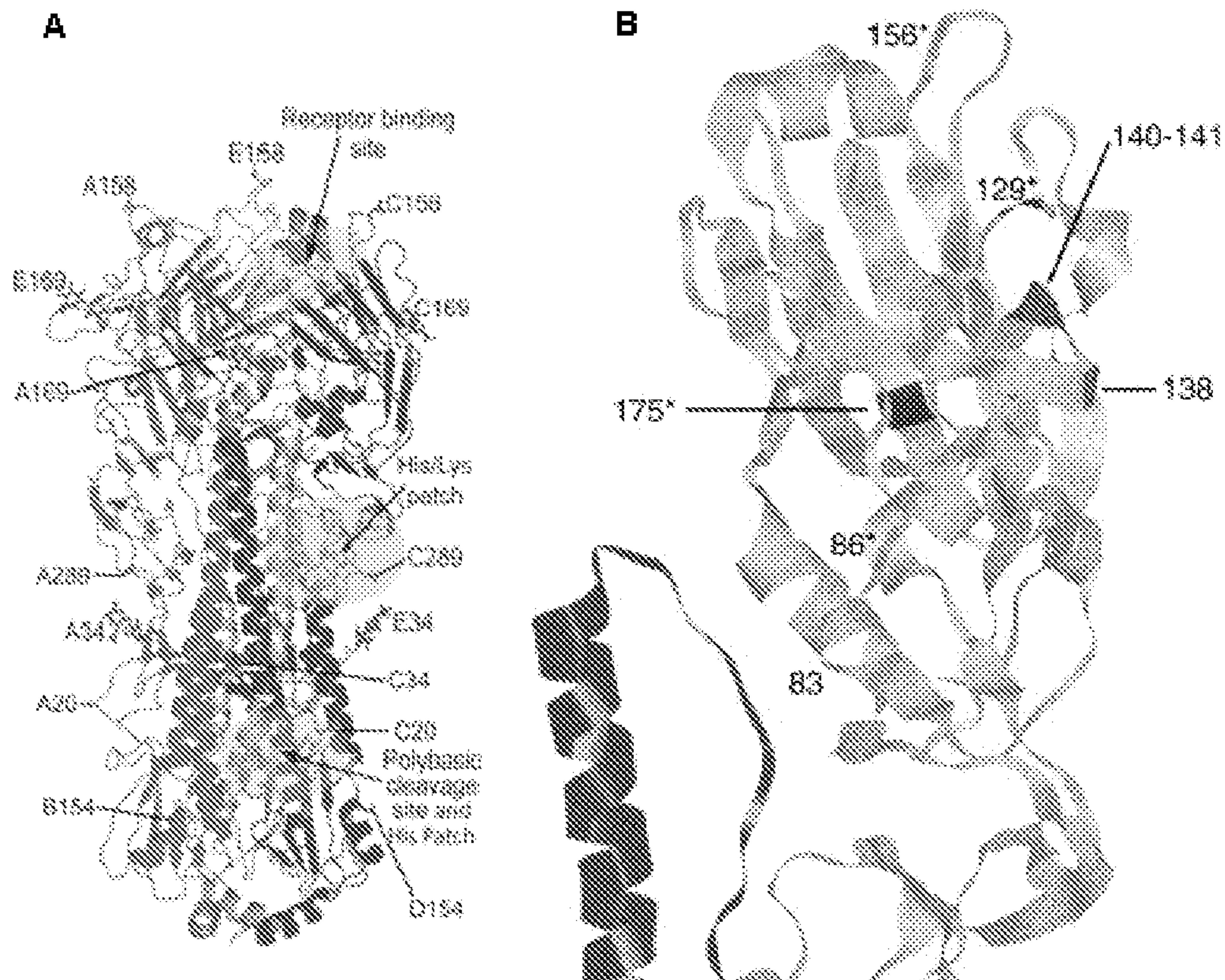
Figure 1. A, Structural overview of the A/Vietnam 1203/04 trimer, receptor binding site and antigenic variation sites are highlighted on the monomer (cited from Stevens, 2006). B, Location of amino acid residues in the HA of H5N1 influenza viruses that are under positive selection (cited from Smith, 2006).
